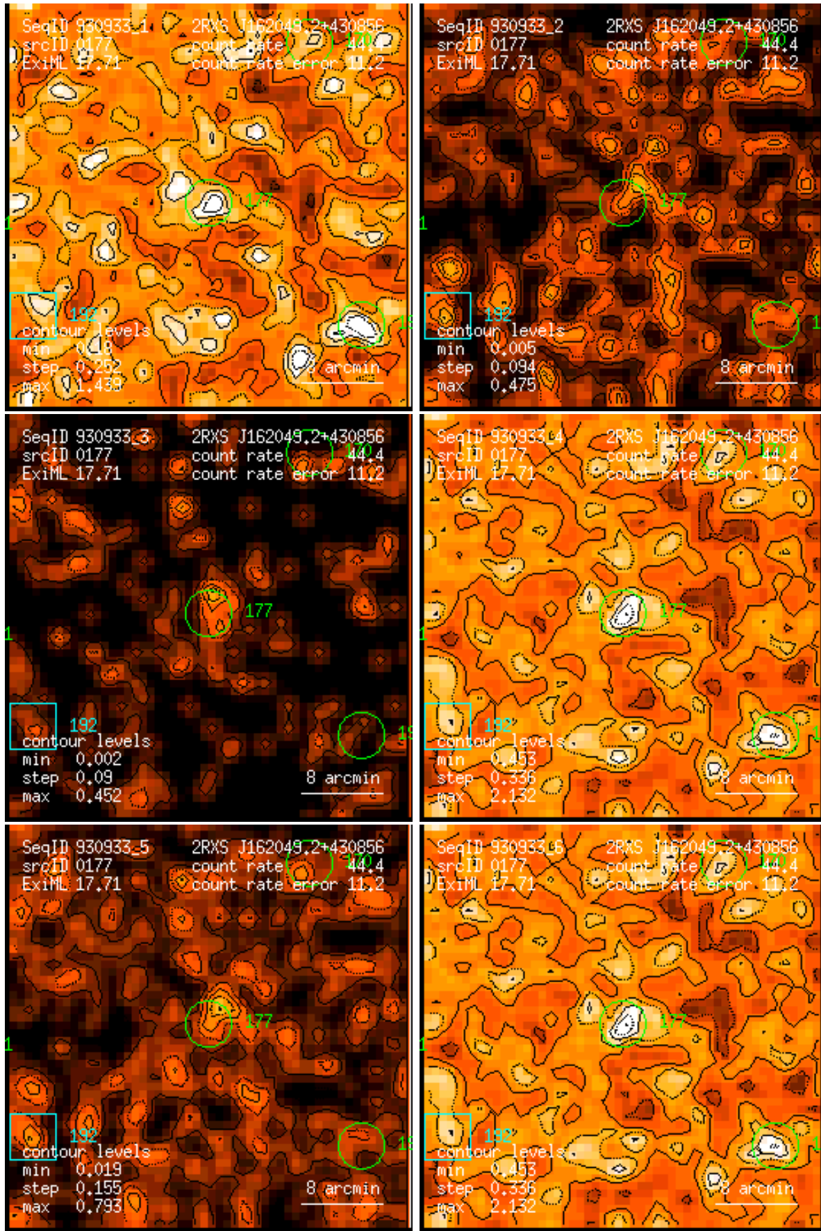
Figure 177: RASS 930933: detection 0177: band rate images, Gaussian filter: (1) PSPC channels 11 – 41, (2) 52 – 90, (3) 91 – 201, (4) 11 – 235, (5) 52 – 201, (6) 11 – 201. Broad band rates in counts/ks. Band rate contour levels in counts/ks/arcmin 2 .
