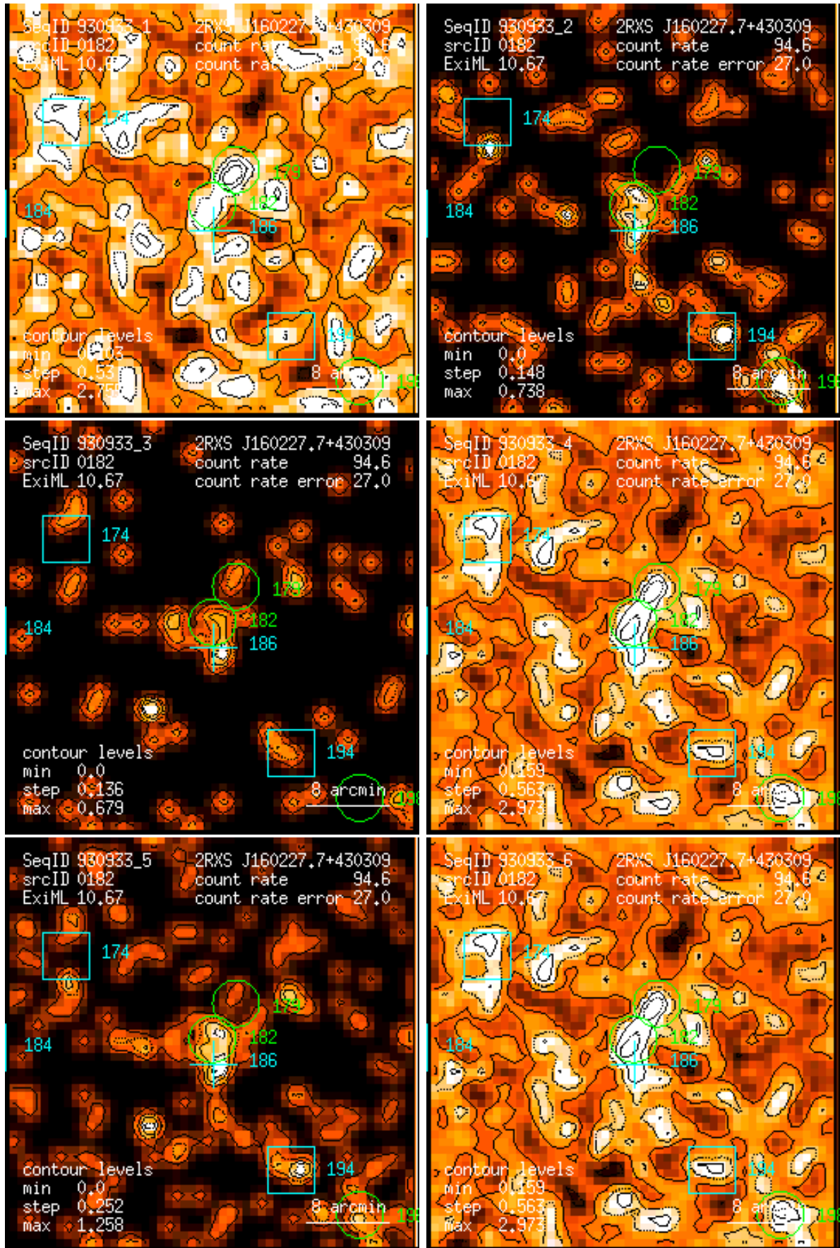
Figure 182: RASS 930933: detection 0182: band rate images, Gaussian filter: (1) PSPC channels 11 – 41, (2) 52 – 90, (3) 91 – 201, (4) 11 – 235, (5) 52 – 201, (6) 11 – 201. Broad band rates in counts/ks. Band rate contour levels in counts/ks/arcmin 2 .
