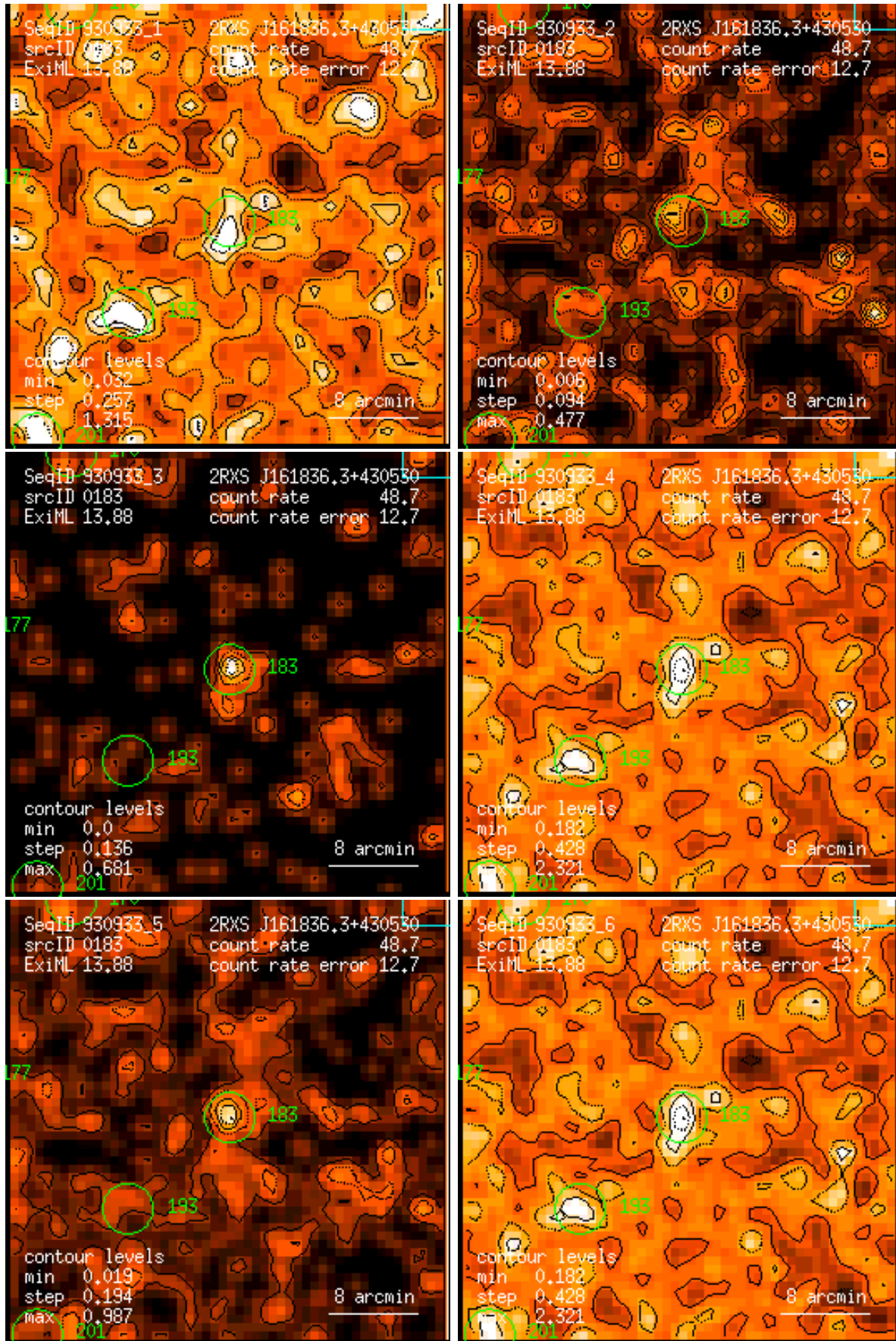
Figure 183: RASS 930933: detection 0183: band rate images, Gaussian filter: (1) PSPC channels 11 – 41, (2) 52 – 90, (3) 91 – 201, (4) 11 – 235, (5) 52 – 201, (6) 11 – 201. Broad band rates in counts/ks. Band rate contour levels in counts/ks/arcmin 2 .
