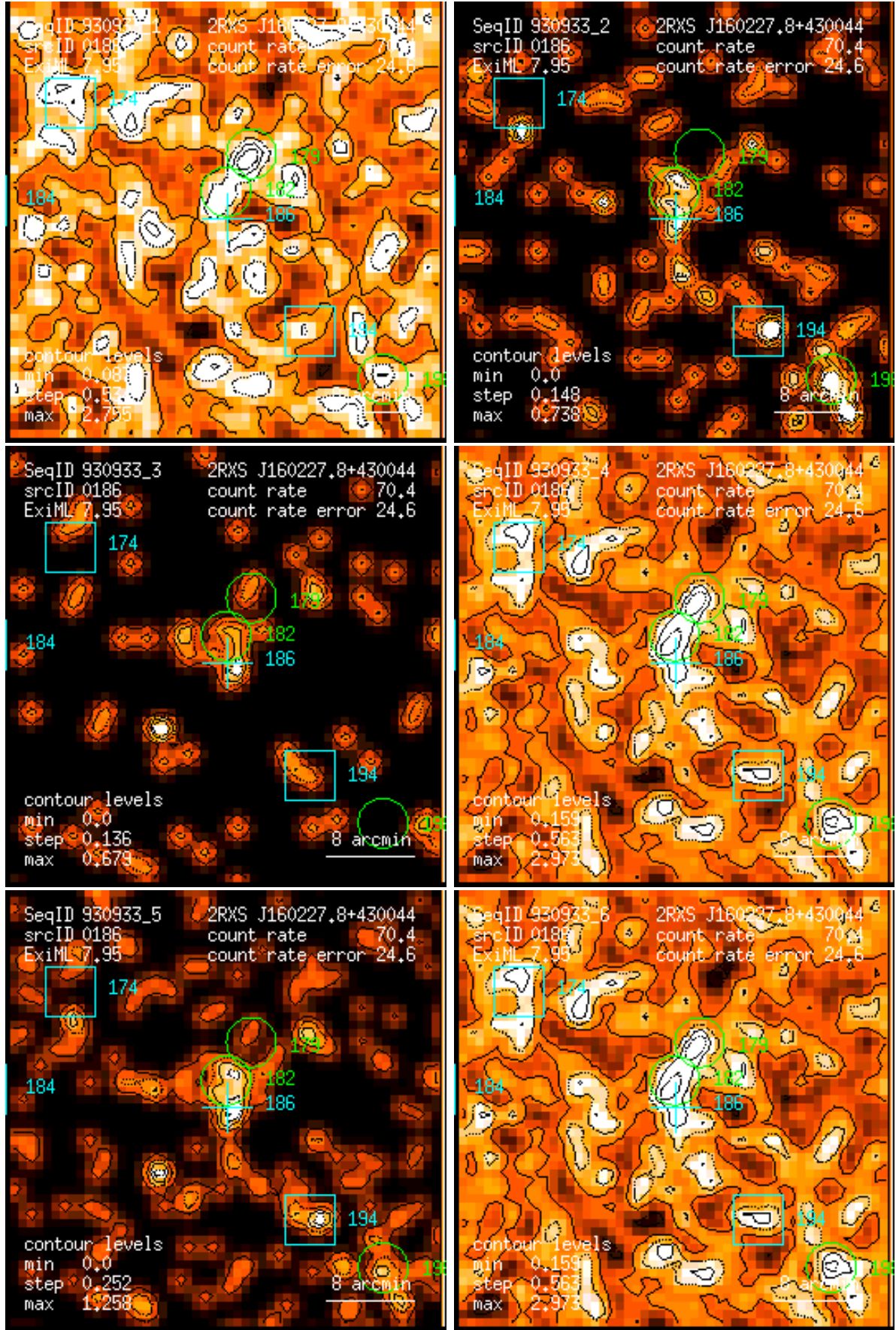
Figure 186: RASS 930933: detection 0186: band rate images, Gaussian filter: (1) PSPC channels 11 – 41, (2) 52 – 90, (3) 91 – 201, (4) 11 – 235, (5) 52 – 201, (6) 11 – 201. Broad band rates in counts/ks. Band rate contour levels in counts/ks/arcmin 2 .
