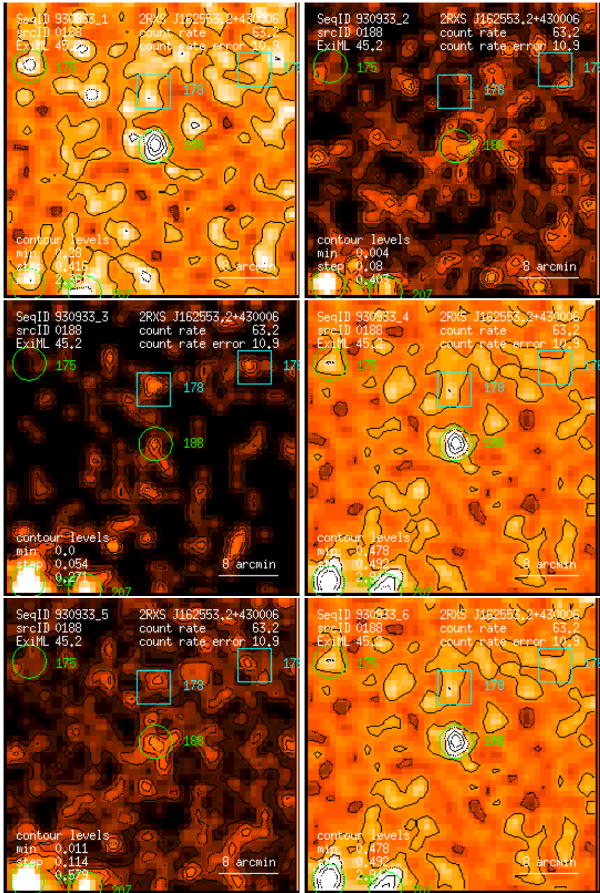
Figure 188: RASS 930933: detection 0188: band rate images, Gaussian filter: (1) PSPC channels 11 – 41, (2) 52 – 90, (3) 91 – 201, (4) 11 – 235, (5) 52 – 201, (6) 11 – 201. Broad band rates in counts/ks. Band rate contour levels in counts/ks/arcmin 2 .
