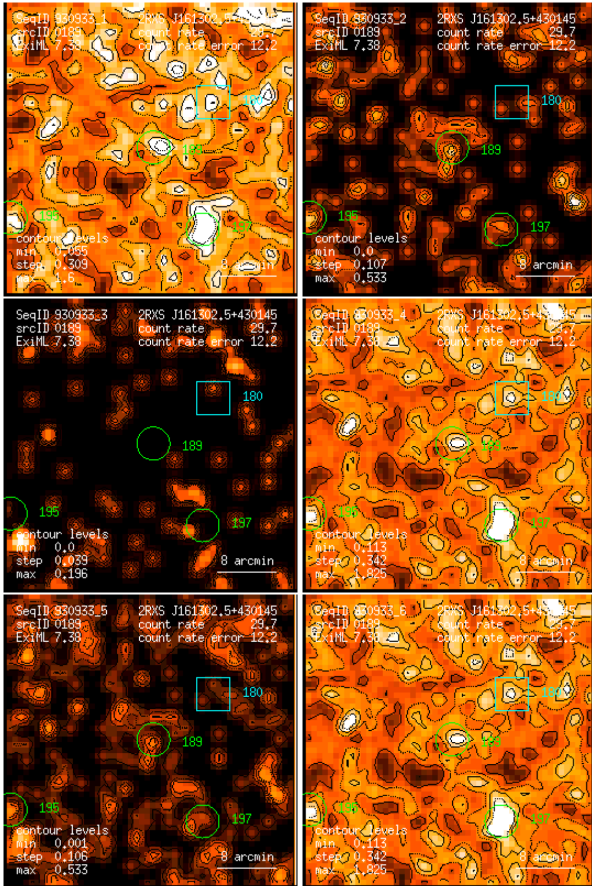
Figure 189: RASS 930933: detection 0189: band rate images, Gaussian filter: (1) PSPC channels 11 – 41, (2) 52 – 90, (3) 91 – 201, (4) 11 – 235, (5) 52 – 201, (6) 11 – 201. Broad band rates in counts/ks. Band rate contour levels in counts/ks/arcmin 2 .
