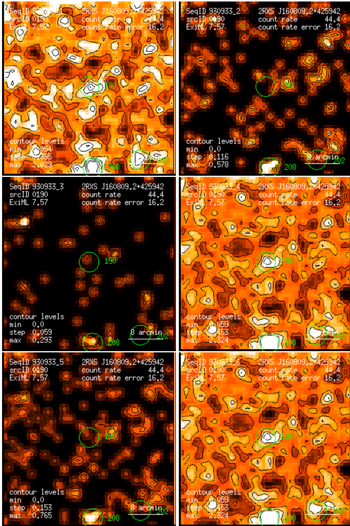
Figure 190: RASS 930933: detection 0190: band rate images, Gaussian filter: (1) PSPC channels 11 – 41, (2) 52 – 90, (3) 91 – 201, (4) 11 – 235, (5) 52 – 201, (6) 11 – 201. Broad band rates in counts/ks. Band rate contour levels in counts/ks/arcmin 2 .
