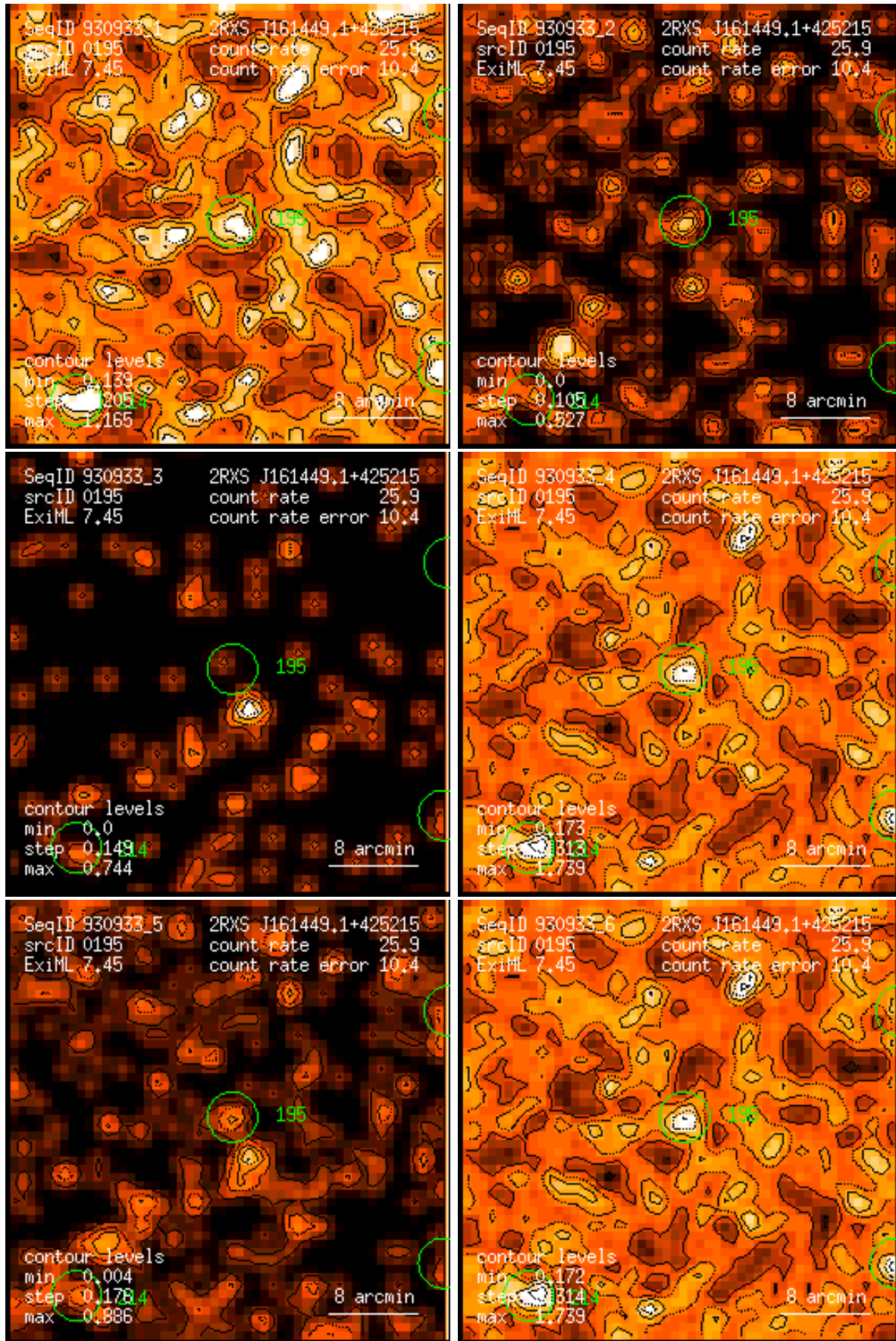
Figure 195: RASS 930933: detection 0195: band rate images, Gaussian filter: (1) PSPC channels 11 – 41, (2) 52 – 90, (3) 91 – 201, (4) 11 – 235, (5) 52 – 201, (6) 11 – 201. Broad band rates in counts/ks. Band rate contour levels in counts/ks/arcmin 2 .
