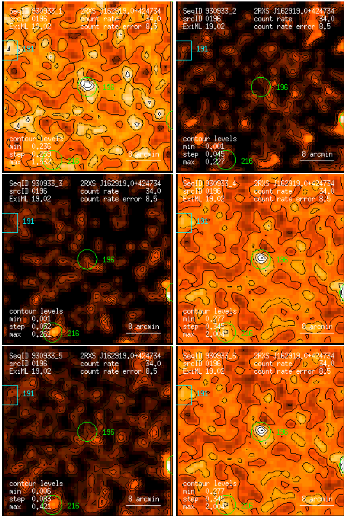
Figure 196: RASS 930933: detection 0196: band rate images, Gaussian filter: (1) PSPC channels 11 – 41, (2) 52 – 90, (3) 91 – 201, (4) 11 – 235, (5) 52 – 201, (6) 11 – 201. Broad band rates in counts/ks. Band rate contour levels in counts/ks/arcmin 2 .
