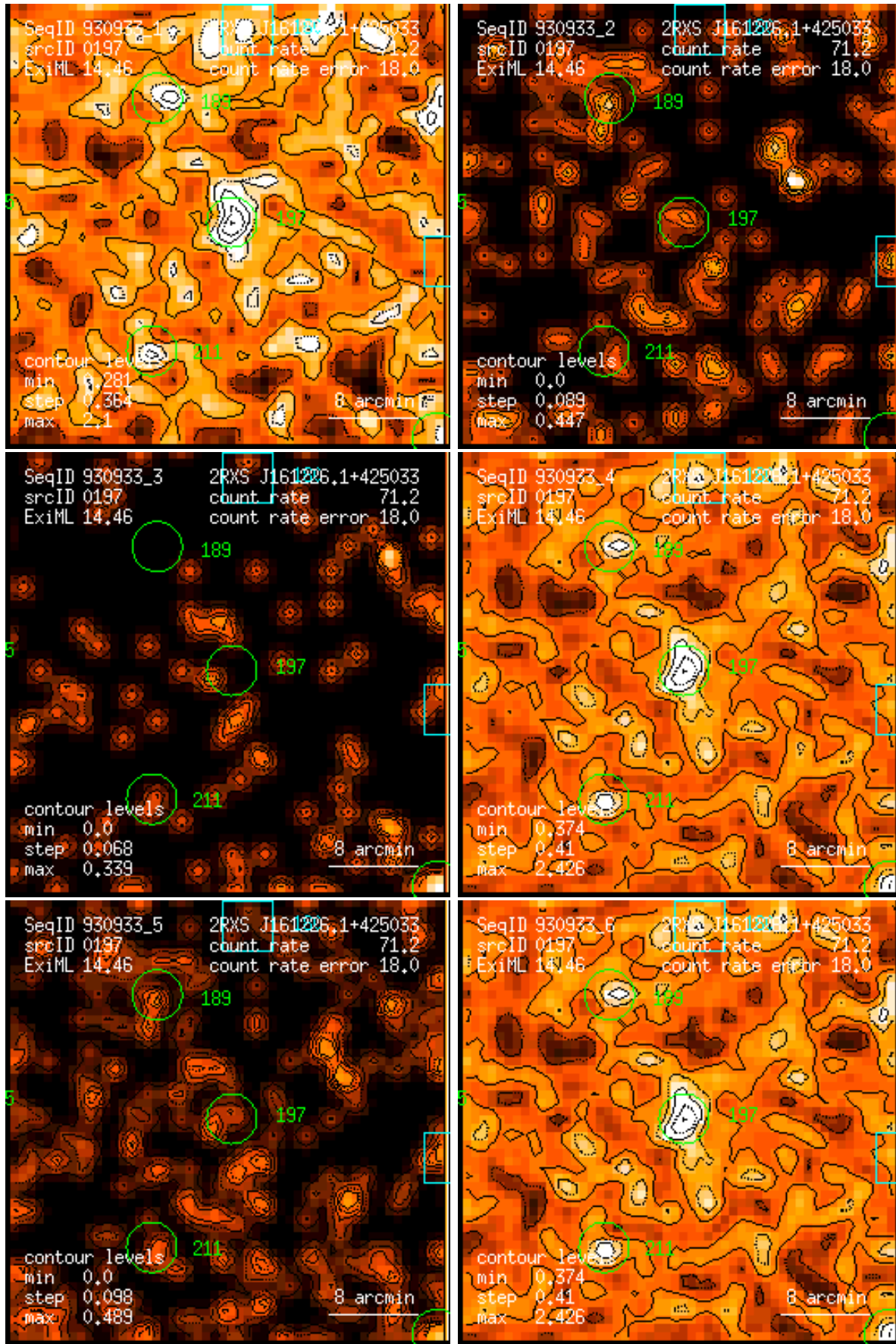
Figure 197: RASS 930933: detection 0197: band rate images, Gaussian filter: (1) PSPC channels 11 – 41, (2) 52 – 90, (3) 91 – 201, (4) 11 – 235, (5) 52 – 201, (6) 11 – 201. Broad band rates in counts/ks. Band rate contour levels in counts/ks/arcmin 2 .
