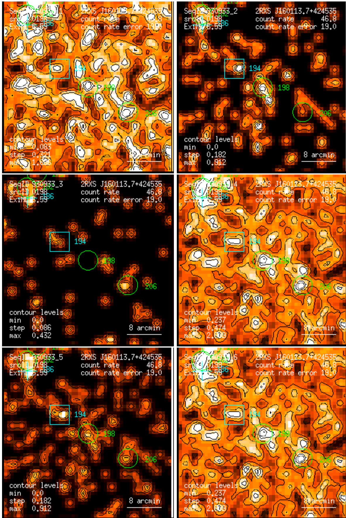
Figure 198: RASS 930933: detection 0198: band rate images, Gaussian filter: (1) PSPC channels 11 – 41, (2) 52 – 90, (3) 91 – 201, (4) 11 – 235, (5) 52 – 201, (6) 11 – 201. Broad band rates in counts/ks. Band rate contour levels in counts/ks/arcmin 2 .
