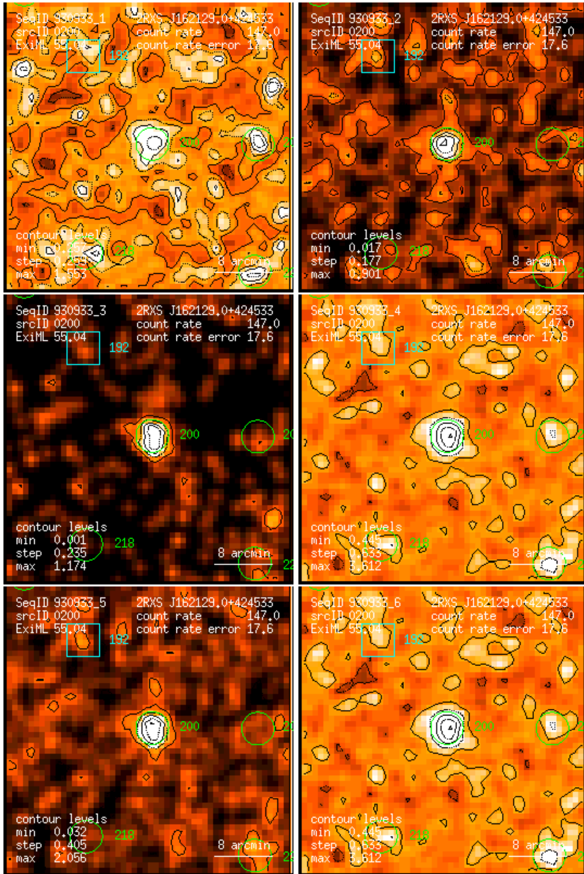
Figure 200: RASS 930933: detection 0200: band rate images, Gaussian filter: (1) PSPC channels 11 – 41, (2) 52 – 90, (3) 91 – 201, (4) 11 – 235, (5) 52 – 201, (6) 11 – 201. Broad band rates in counts/ks. Band rate contour levels in counts/ks/arcmin 2 .
