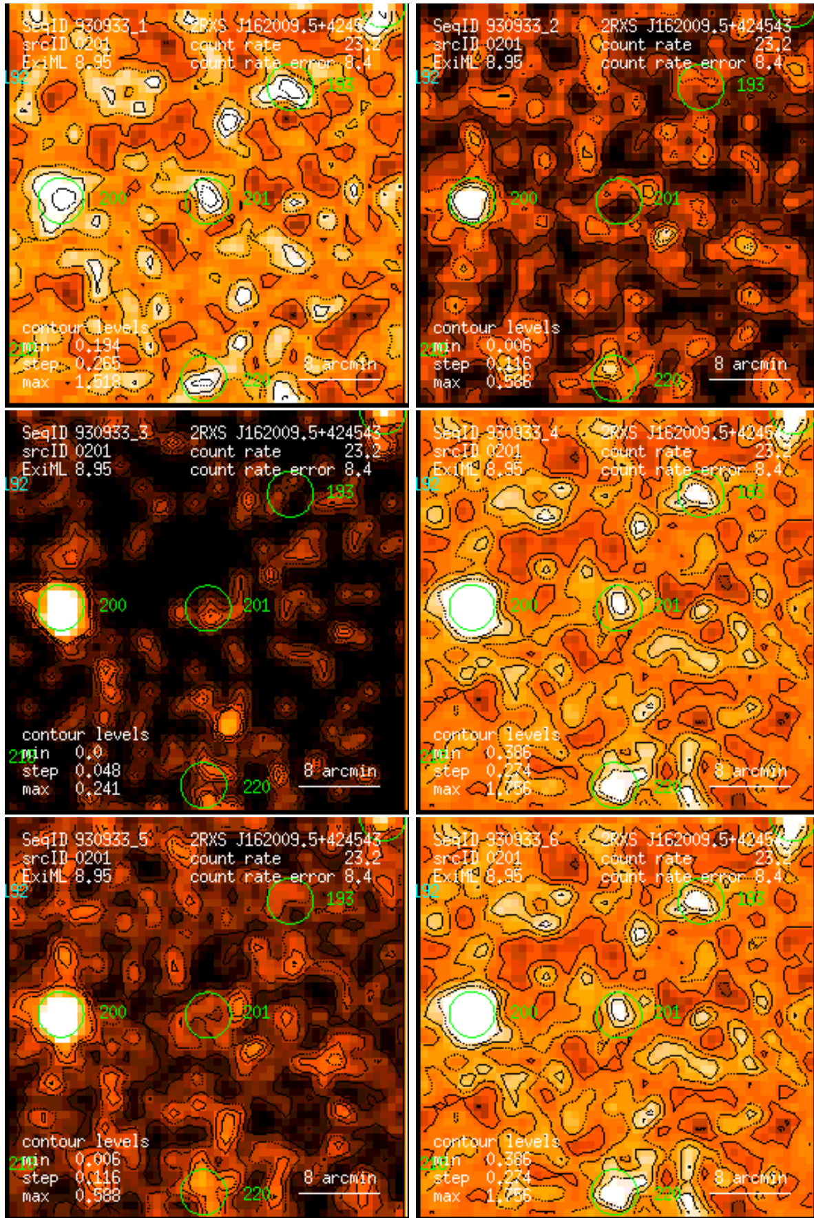
Figure 201: RASS 930933: detection 0201: band rate images, Gaussian filter: (1) PSPC channels 11 – 41, (2) 52 – 90, (3) 91 – 201, (4) 11 – 235, (5) 52 – 201, (6) 11 – 201. Broad band rates in counts/ks. Band rate contour levels in counts/ks/arcmin 2 .
