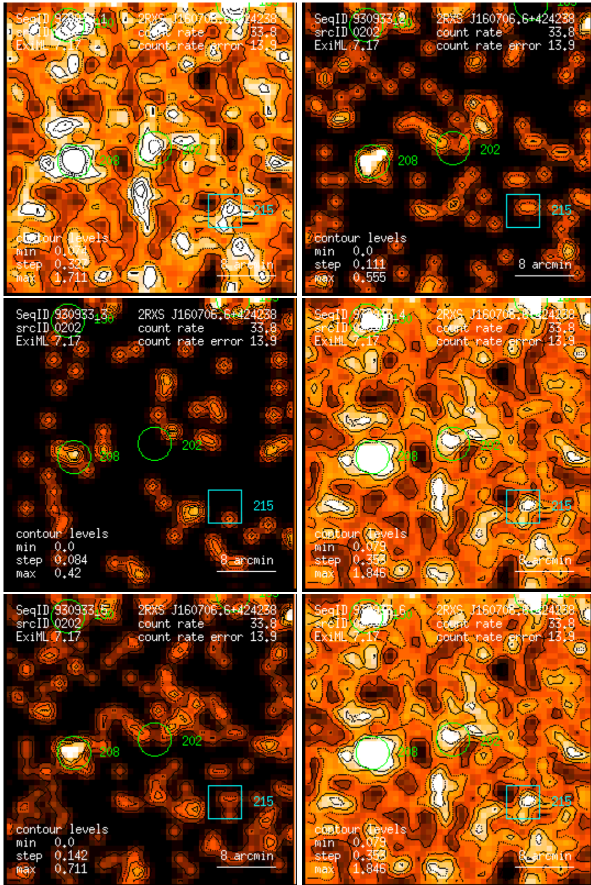
Figure 202: RASS 930933: detection 0202: band rate images, Gaussian filter: (1) PSPC channels 11 – 41, (2) 52 – 90, (3) 91 – 201, (4) 11 – 235, (5) 52 – 201, (6) 11 – 201. Broad band rates in counts/ks. Band rate contour levels in counts/ks/arcmin 2 .
