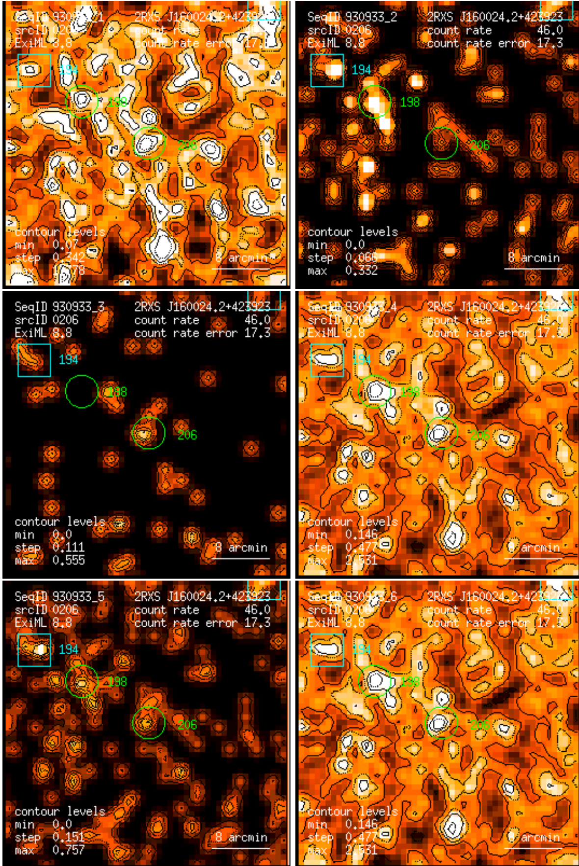
Figure 206: RASS 930933: detection 0206: band rate images, Gaussian filter: (1) PSPC channels 11 – 41, (2) 52 – 90, (3) 91 – 201, (4) 11 – 235, (5) 52 – 201, (6) 11 – 201. Broad band rates in counts/ks. Band rate contour levels in counts/ks/arcmin 2 .
