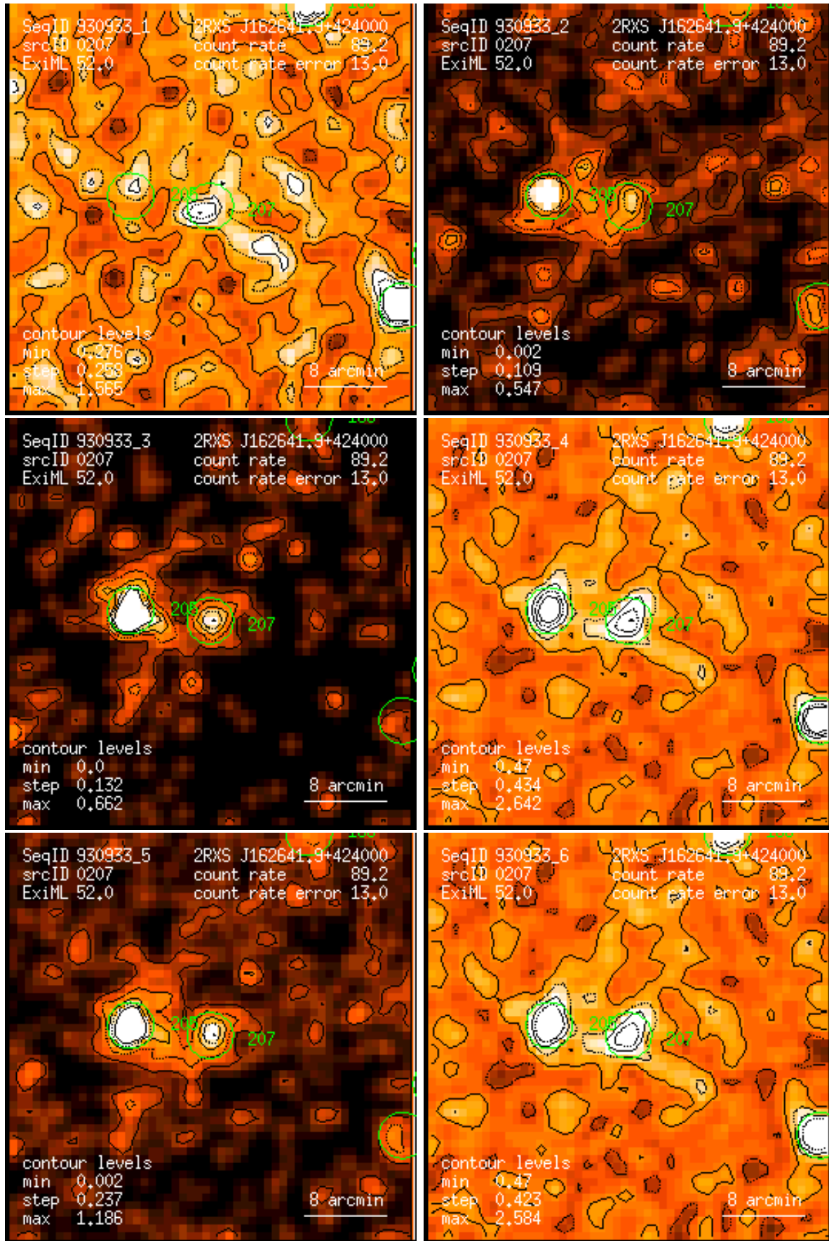
Figure 207: RASS 930933: detection 0207: band rate images, Gaussian filter: (1) PSPC channels 11 – 41, (2) 52 – 90, (3) 91 – 201, (4) 11 – 235, (5) 52 – 201, (6) 11 – 201. Broad band rates in counts/ks. Band rate contour levels in counts/ks/arcmin 2 .
