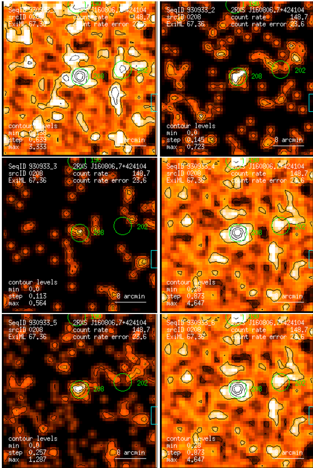
Figure 208: RASS 930933: detection 0208: band rate images, Gaussian filter: (1) PSPC channels 11 – 41, (2) 52 – 90, (3) 91 – 201, (4) 11 – 235, (5) 52 – 201, (6) 11 – 201. Broad band rates in counts/ks. Band rate contour levels in counts/ks/arcmin 2 .
