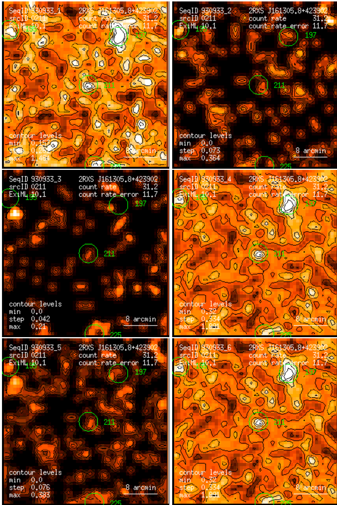
Figure 211: RASS 930933: detection 0211: band rate images, Gaussian filter: (1) PSPC channels 11 – 41, (2) 52 – 90, (3) 91 – 201, (4) 11 – 235, (5) 52 – 201, (6) 11 – 201. Broad band rates in counts/ks. Band rate contour levels in counts/ks/arcmin 2 .
