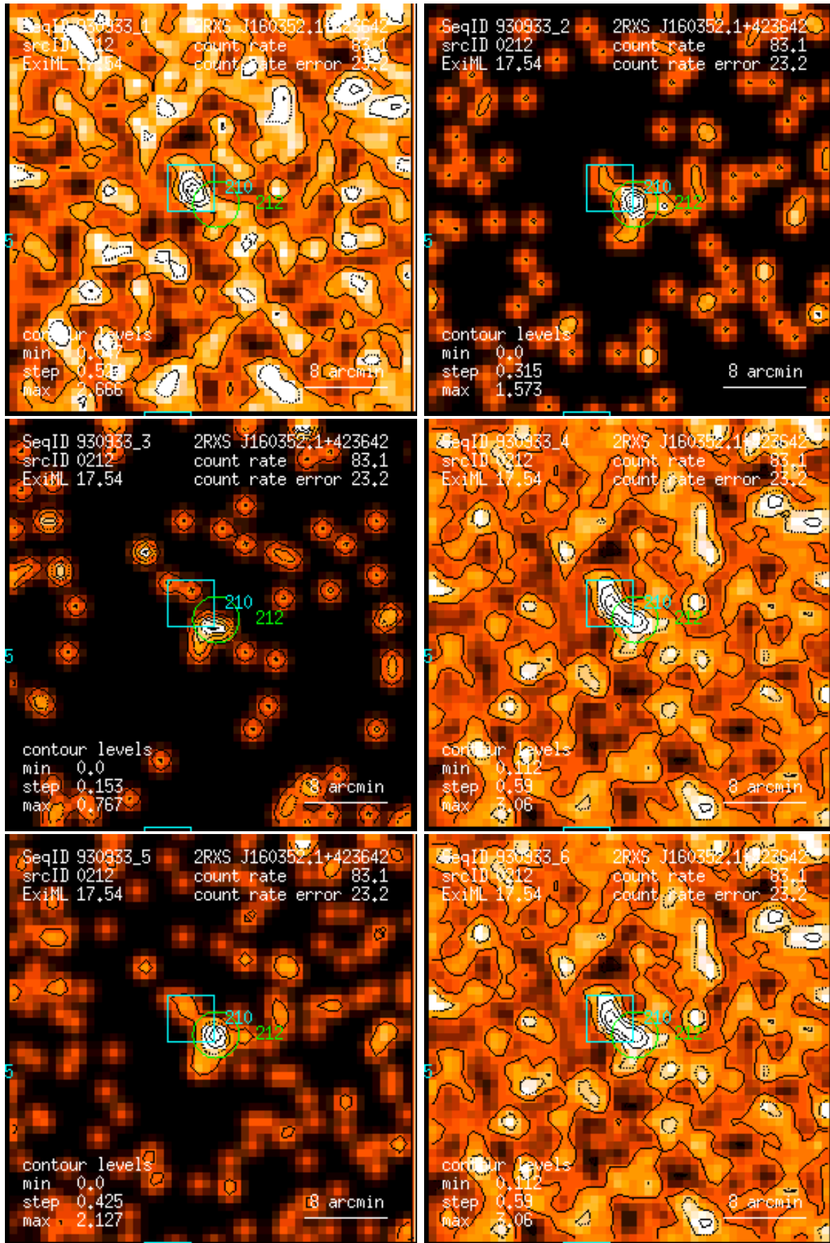
Figure 212: RASS 930933: detection 0212: band rate images, Gaussian filter: (1) PSPC channels 11 – 41, (2) 52 – 90, (3) 91 – 201, (4) 11 – 235, (5) 52 – 201, (6) 11 – 201. Broad band rates in counts/ks. Band rate contour levels in counts/ks/arcmin 2 .
