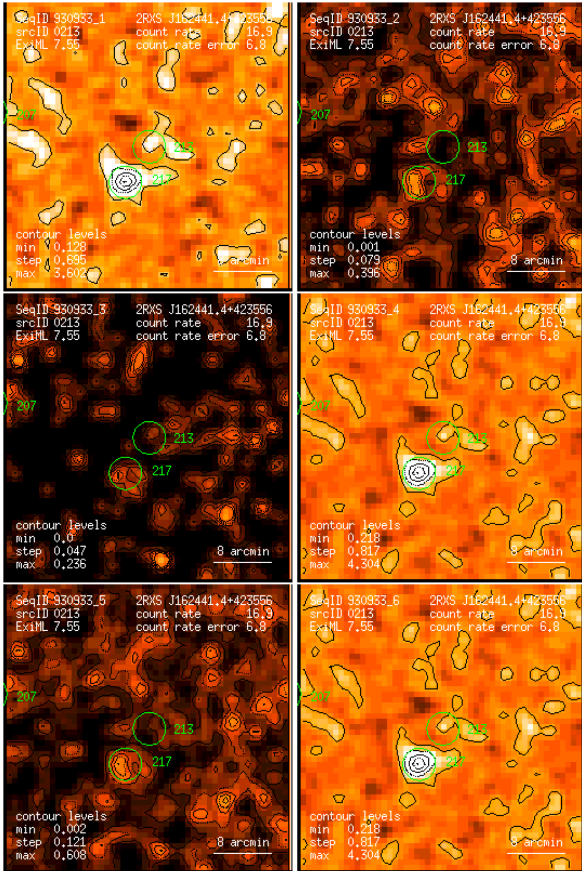
Figure 213: RASS 930933: detection 0213: band rate images, Gaussian filter: (1) PSPC channels 11 – 41, (2) 52 – 90, (3) 91 – 201, (4) 11 – 235, (5) 52 – 201, (6) 11 – 201. Broad band rates in counts/ks. Band rate contour levels in counts/ks/arcmin 2 .
