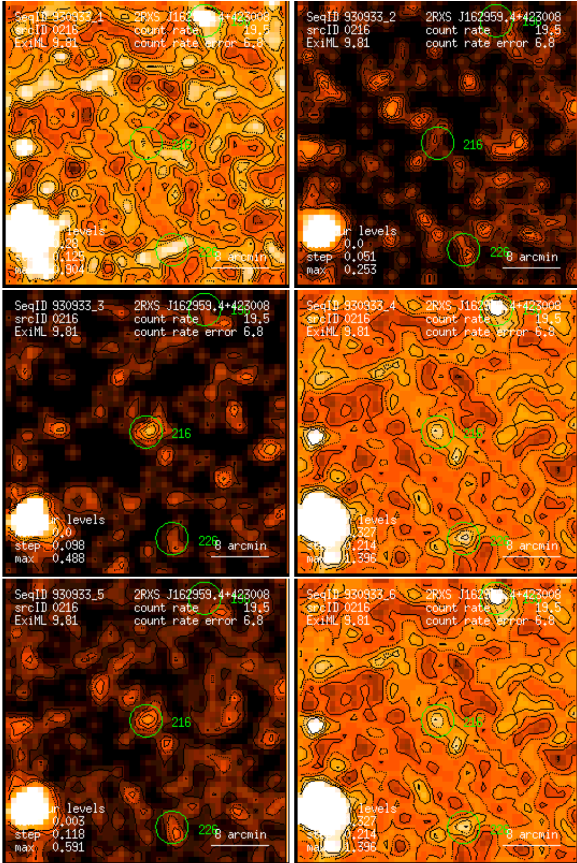
Figure 216: RASS 930933: detection 0216: band rate images, Gaussian filter: (1) PSPC channels 11 – 41, (2) 52 – 90, (3) 91 – 201, (4) 11 – 235, (5) 52 – 201, (6) 11 – 201. Broad band rates in counts/ks. Band rate contour levels in counts/ks/arcmin 2 .
