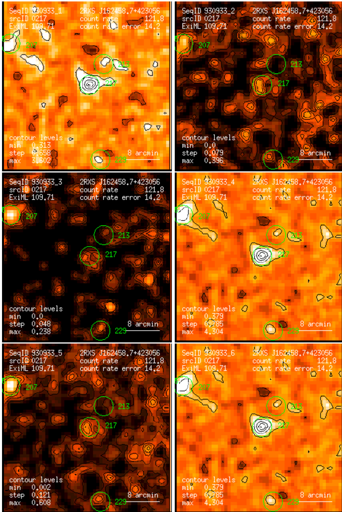
Figure 217: RASS 930933: detection 0217: band rate images, Gaussian filter: (1) PSPC channels 11 – 41, (2) 52 – 90, (3) 91 – 201, (4) 11 – 235, (5) 52 – 201, (6) 11 – 201. Broad band rates in counts/ks. Band rate contour levels in counts/ks/arcmin 2 .
