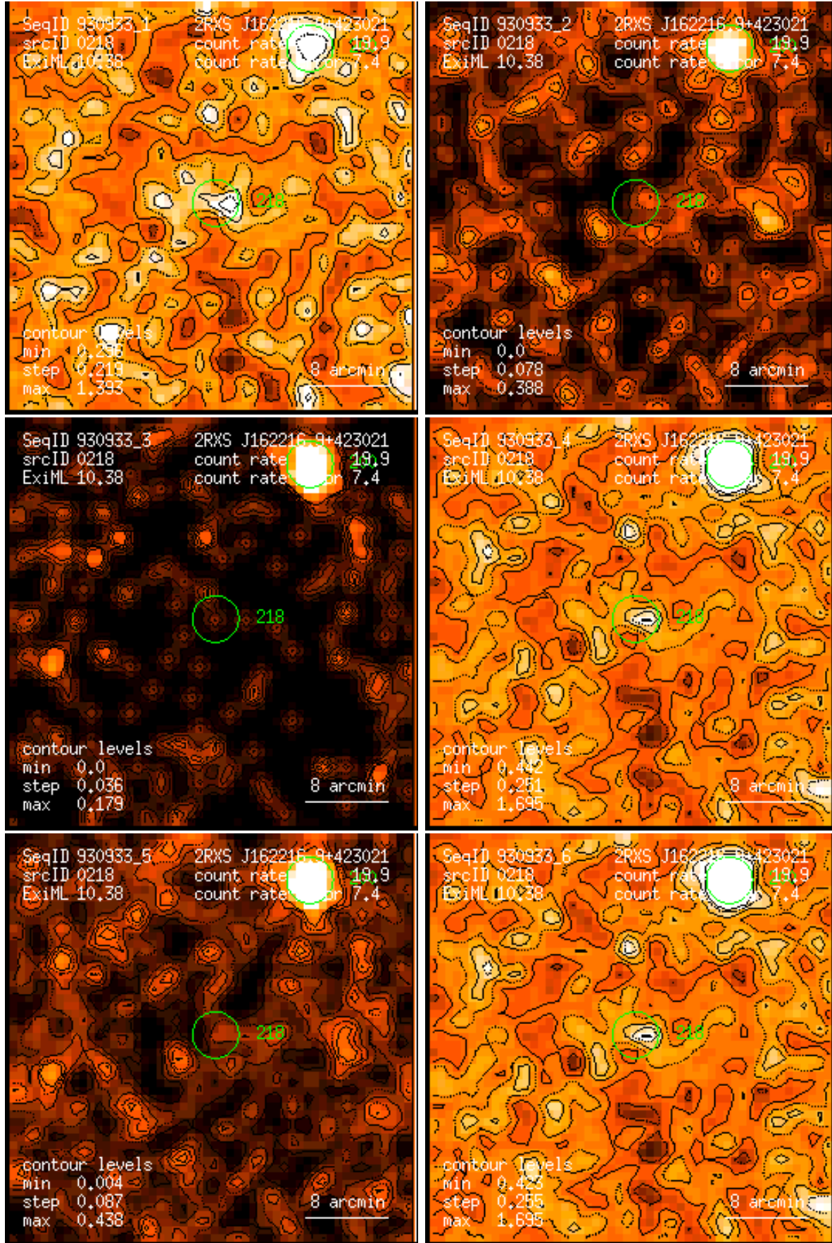
Figure 218: RASS 930933: detection 0218: band rate images, Gaussian filter: (1) PSPC channels 11 – 41, (2) 52 – 90, (3) 91 – 201, (4) 11 – 235, (5) 52 – 201, (6) 11 – 201. Broad band rates in counts/ks. Band rate contour levels in counts/ks/arcmin 2 .
