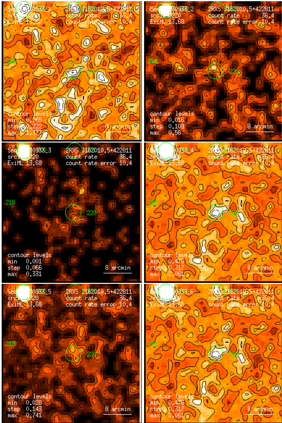
Figure 220: RASS 930933: detection 0220: band rate images, Gaussian filter: (1) PSPC channels 11 – 41, (2) 52 – 90, (3) 91 – 201, (4) 11 – 235, (5) 52 – 201, (6) 11 – 201. Broad band rates in counts/ks. Band rate contour levels in counts/ks/arcmin 2 .
