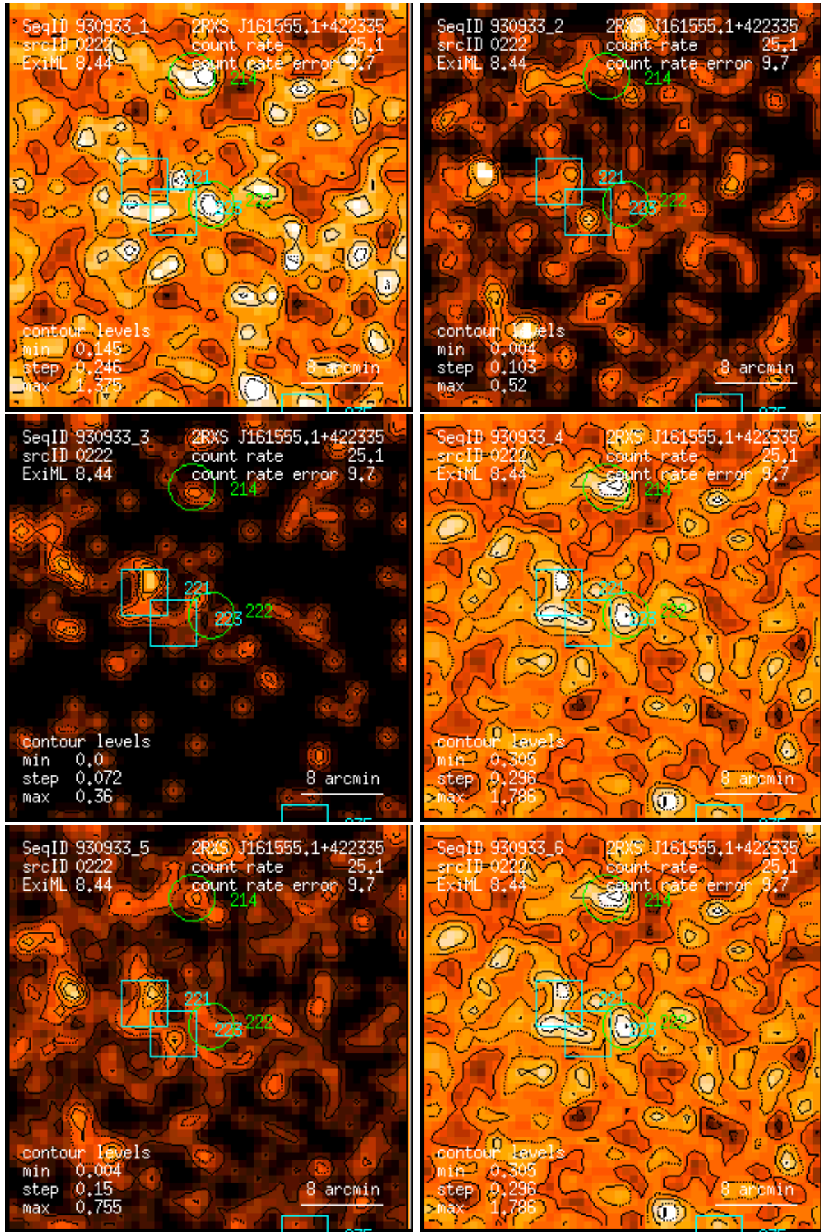
Figure 222: RASS 930933: detection 0222: band rate images, Gaussian filter: (1) PSPC channels 11 – 41, (2) 52 – 90, (3) 91 – 201, (4) 11 – 235, (5) 52 – 201, (6) 11 – 201. Broad band rates in counts/ks. Band rate contour levels in counts/ks/arcmin 2 .
