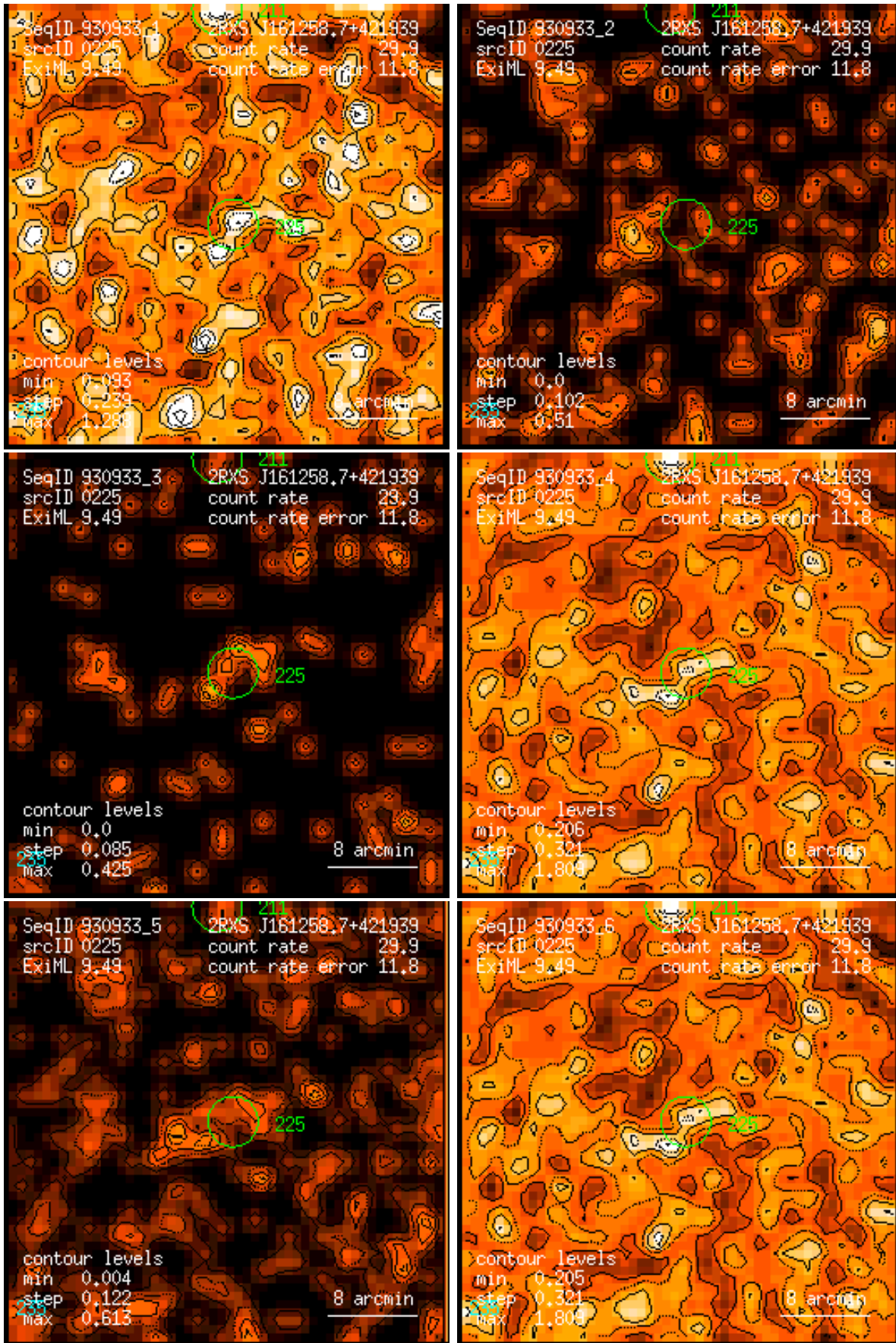
Figure 225: RASS 930933: detection 0225: band rate images, Gaussian filter: (1) PSPC channels 11 – 41, (2) 52 – 90, (3) 91 – 201, (4) 11 – 235, (5) 52 – 201, (6) 11 – 201. Broad band rates in counts/ks. Band rate contour levels in counts/ks/arcmin 2 .
