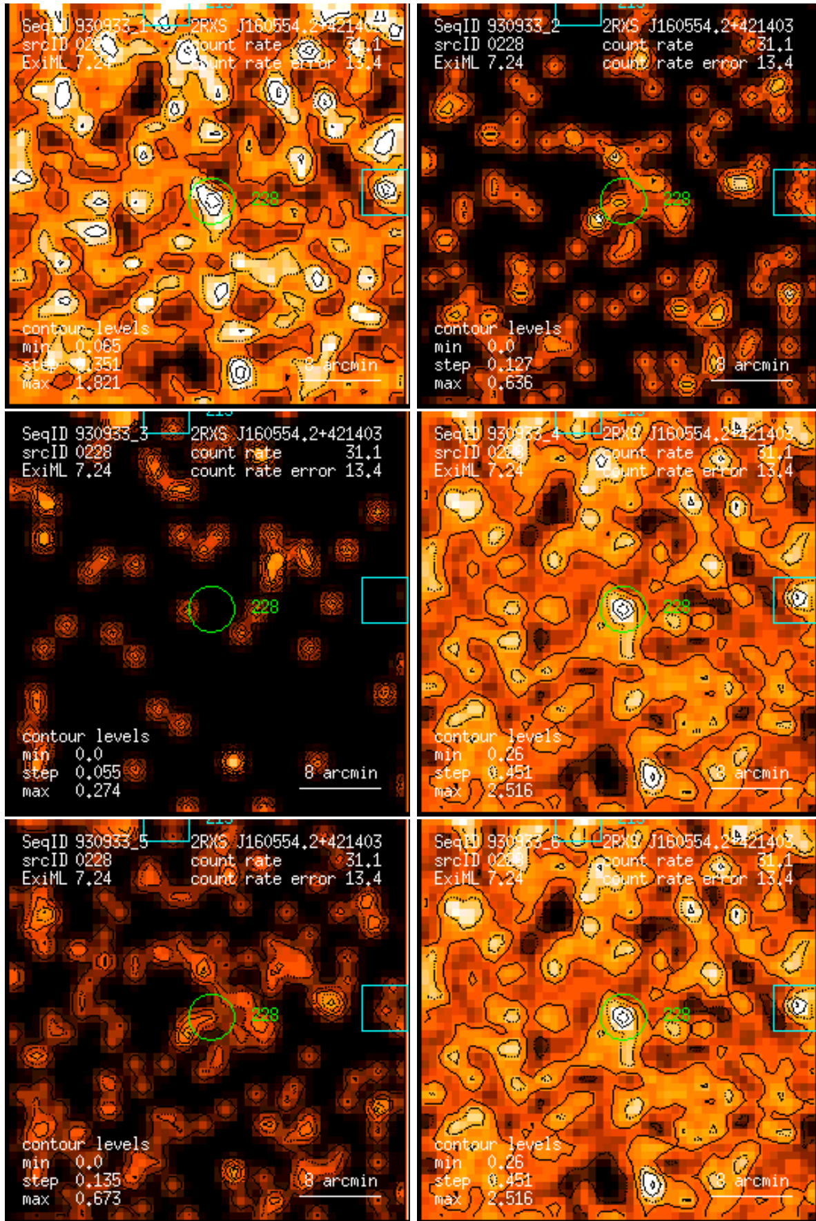
Figure 228: RASS 930933: detection 0228: band rate images, Gaussian filter: (1) PSPC channels 11 – 41, (2) 52 – 90, (3) 91 – 201, (4) 11 – 235, (5) 52 – 201, (6) 11 – 201. Broad band rates in counts/ks. Band rate contour levels in counts/ks/arcmin 2 .
