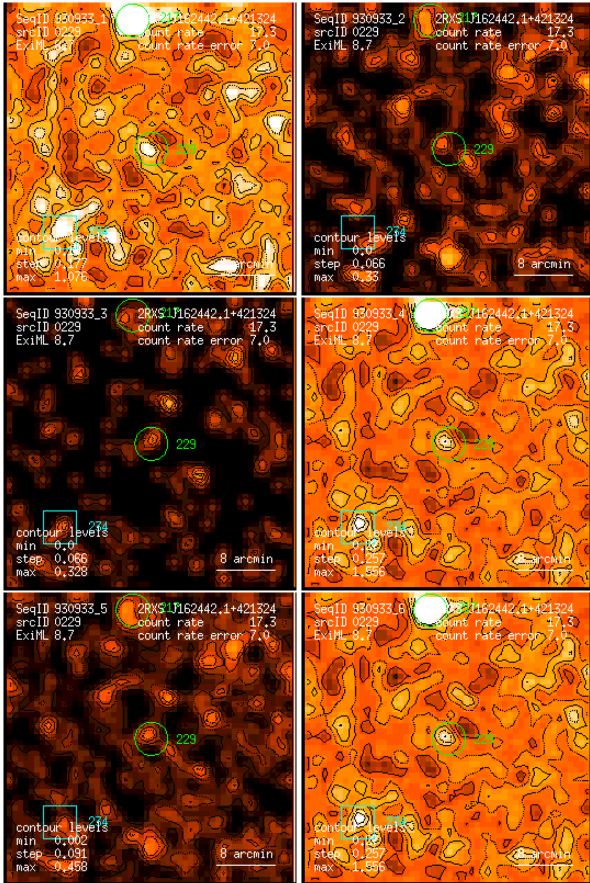
Figure 229: RASS 930933: detection 0229: band rate images, Gaussian filter: (1) PSPC channels 11 – 41, (2) 52 – 90, (3) 91 – 201, (4) 11 – 235, (5) 52 – 201, (6) 11 – 201. Broad band rates in counts/ks. Band rate contour levels in counts/ks/arcmin 2 .
