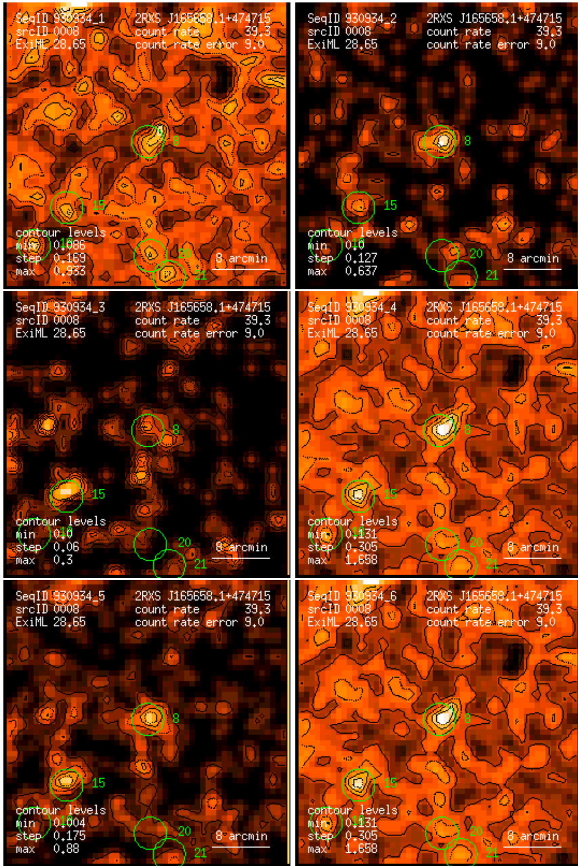
Figure 8: RASS 930934: detection 0008: band rate images, Gaussian filter: (1) PSPC channels 11 – 41, (2) 52 – 90, (3) 91 – 201, (4) 11 – 235, (5) 52 – 201, (6) 11 – 201. Broad band rates in counts/ks. Band rate contour levels in counts/ks/arcmin 2 .
