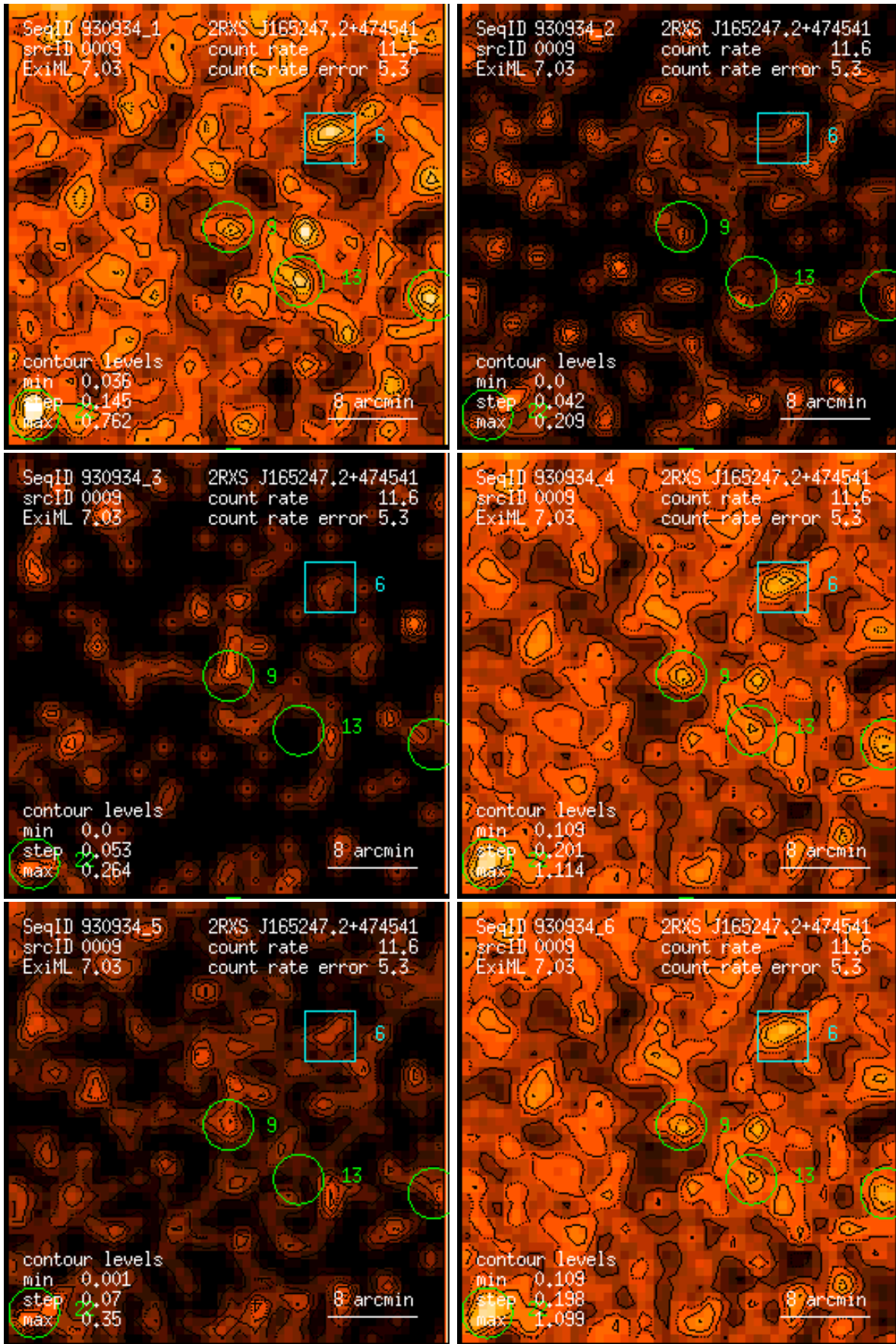
Figure 9: RASS 930934: detection 0009: band rate images, Gaussian filter: (1) PSPC channels 11 – 41, (2) 52 – 90, (3) 91 – 201, (4) 11 – 235, (5) 52 – 201, (6) 11 – 201. Broad band rates in counts/ks. Band rate contour levels in counts/ks/arcmin 2 .
