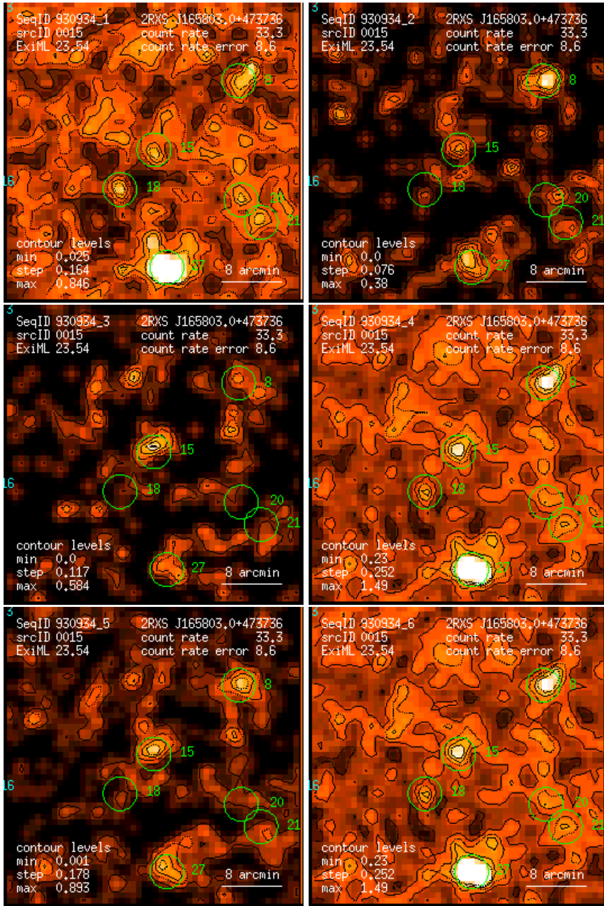
Figure 15: RASS 930934: detection 0015: band rate images, Gaussian filter: (1) PSPC channels 11 – 41, (2) 52 – 90, (3) 91 – 201, (4) 11 – 235, (5) 52 – 201, (6) 11 – 201. Broad band rates in counts/ks. Band rate contour levels in counts/ks/arcmin 2 .
