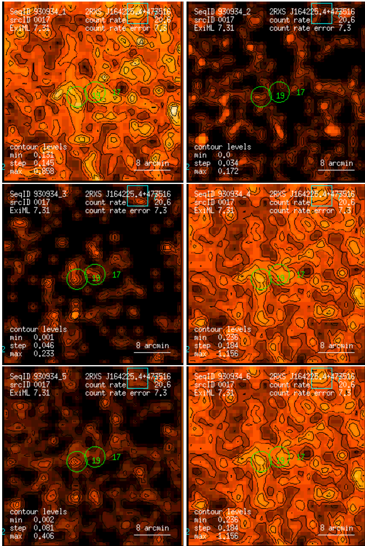
Figure 17: RASS 930934: detection 0017: band rate images, Gaussian filter: (1) PSPC channels 11 – 41, (2) 52 – 90, (3) 91 – 201, (4) 11 – 235, (5) 52 – 201, (6) 11 – 201. Broad band rates in counts/ks. Band rate contour levels in counts/ks/arcmin 2 .
