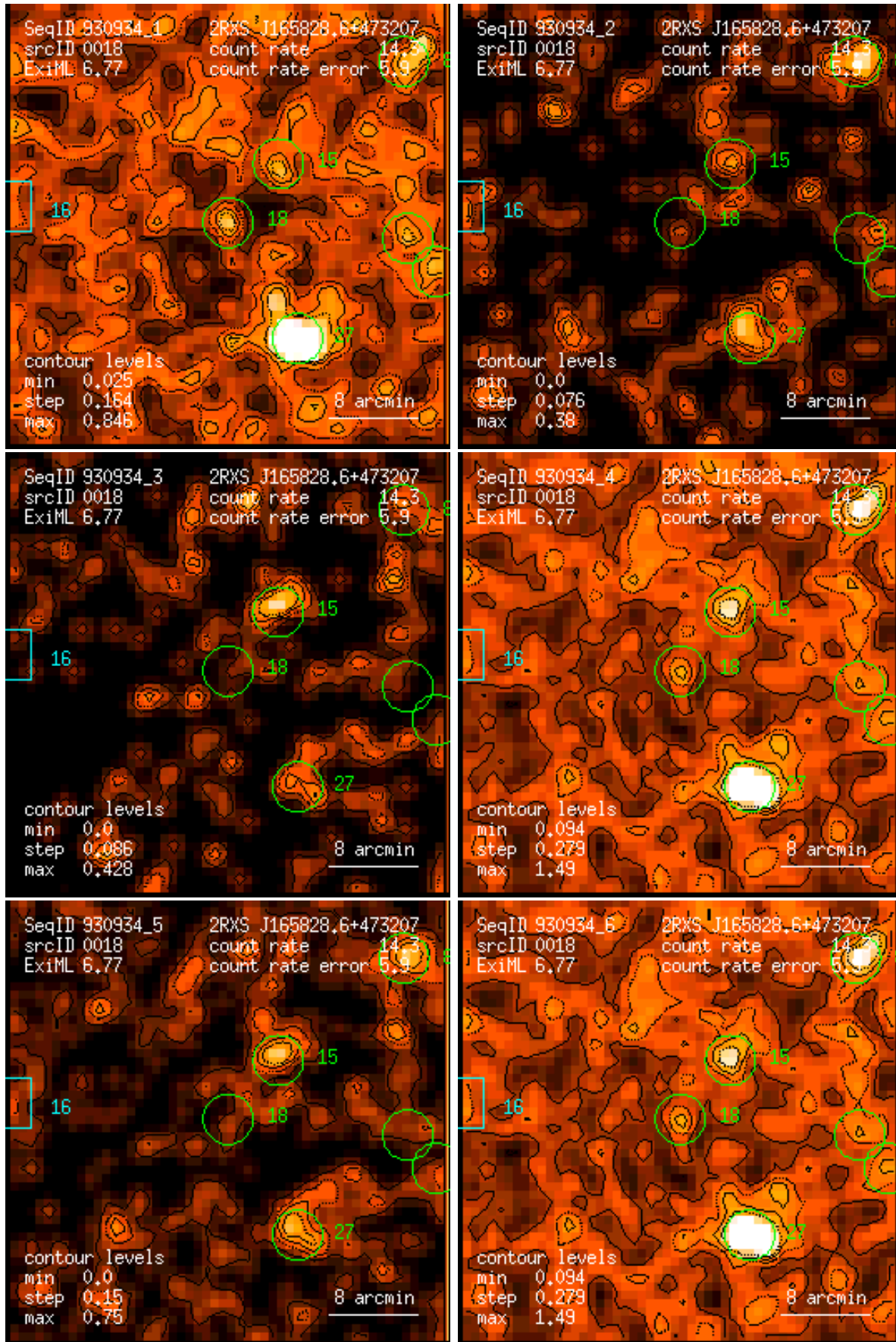
Figure 18: RASS 930934: detection 0018: band rate images, Gaussian filter: (1) PSPC channels 11 – 41, (2) 52 – 90, (3) 91 – 201, (4) 11 – 235, (5) 52 – 201, (6) 11 – 201. Broad band rates in counts/ks. Band rate contour levels in counts/ks/arcmin 2 .
