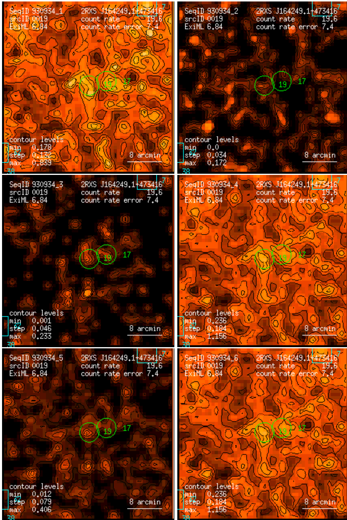
Figure 19: RASS 930934: detection 0019: band rate images, Gaussian filter: (1) PSPC channels 11 – 41, (2) 52 – 90, (3) 91 – 201, (4) 11 – 235, (5) 52 – 201, (6) 11 – 201. Broad band rates in counts/ks. Band rate contour levels in counts/ks/arcmin 2 .
