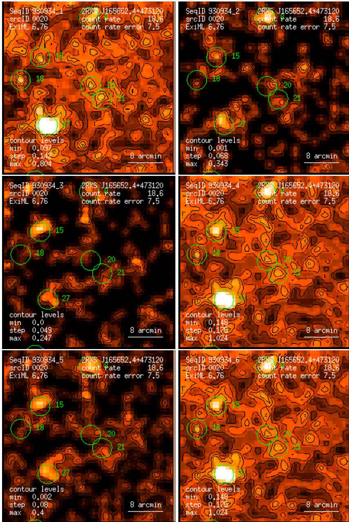
Figure 20: RASS 930934: detection 0020: band rate images, Gaussian filter: (1) PSPC channels 11 – 41, (2) 52 – 90, (3) 91 – 201, (4) 11 – 235, (5) 52 – 201, (6) 11 – 201. Broad band rates in counts/ks. Band rate contour levels in counts/ks/arcmin 2 .
