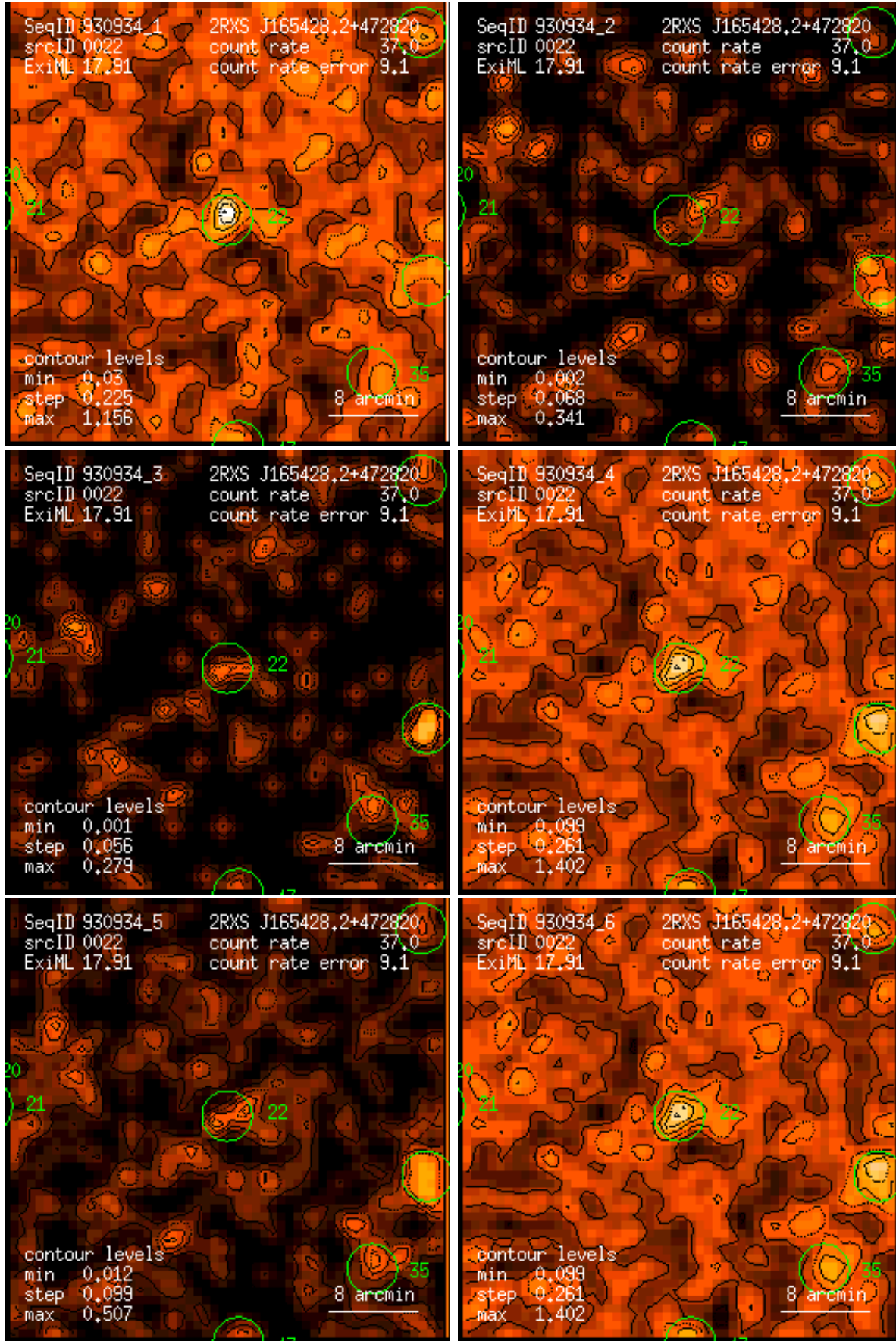
Figure 22: RASS 930934: detection 0022: band rate images, Gaussian filter: (1) PSPC channels 11 – 41, (2) 52 – 90, (3) 91 – 201, (4) 11 – 235, (5) 52 – 201, (6) 11 – 201. Broad band rates in counts/ks. Band rate contour levels in counts/ks/arcmin 2 .
