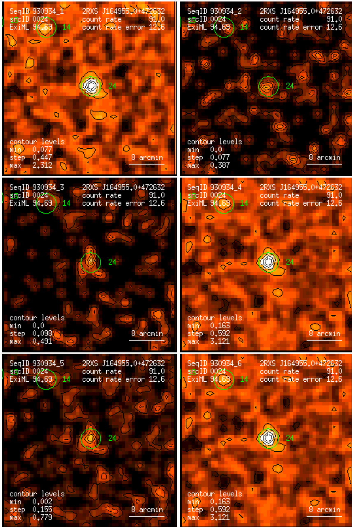
Figure 24: RASS 930934: detection 0024: band rate images, Gaussian filter: (1) PSPC channels 11 – 41, (2) 52 – 90, (3) 91 – 201, (4) 11 – 235, (5) 52 – 201, (6) 11 – 201. Broad band rates in counts/ks. Band rate contour levels in counts/ks/arcmin 2 .
