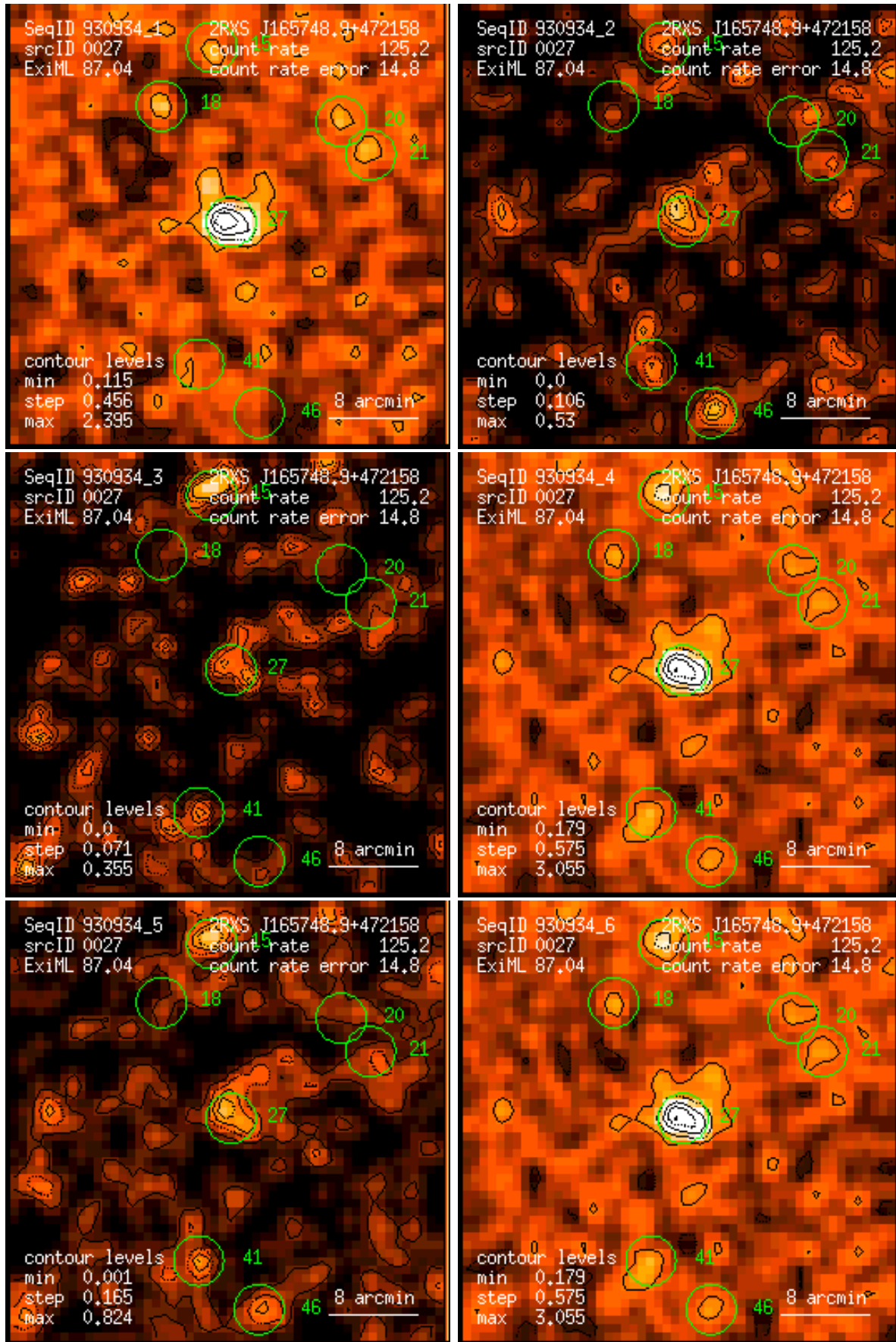
Figure 27: RASS 930934: detection 0027: band rate images, Gaussian filter: (1) PSPC channels 11 – 41, (2) 52 – 90, (3) 91 – 201, (4) 11 – 235, (5) 52 – 201, (6) 11 – 201. Broad band rates in counts/ks. Band rate contour levels in counts/ks/arcmin 2 .
