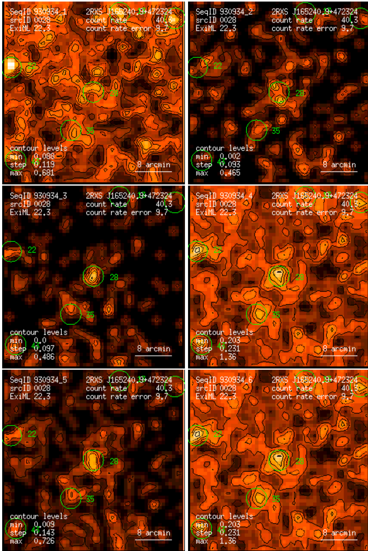
Figure 28: RASS 930934: detection 0028: band rate images, Gaussian filter: (1) PSPC channels 11 – 41, (2) 52 – 90, (3) 91 – 201, (4) 11 – 235, (5) 52 – 201, (6) 11 – 201. Broad band rates in counts/ks. Band rate contour levels in counts/ks/arcmin 2 .
