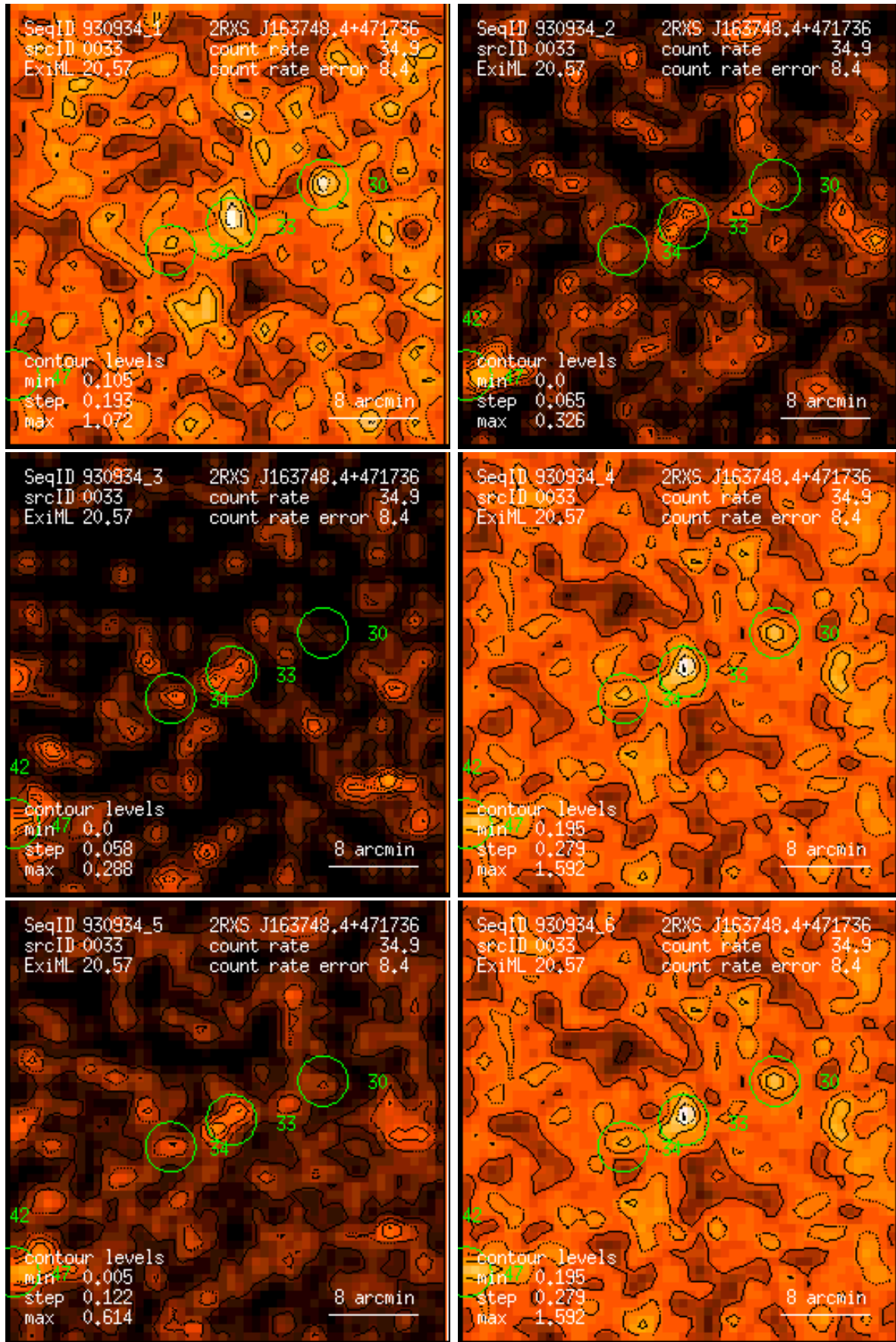
Figure 33: RASS 930934: detection 0033: band rate images, Gaussian filter: (1) PSPC channels 11 – 41, (2) 52 – 90, (3) 91 – 201, (4) 11 – 235, (5) 52 – 201, (6) 11 – 201. Broad band rates in counts/ks. Band rate contour levels in counts/ks/arcmin 2 .
