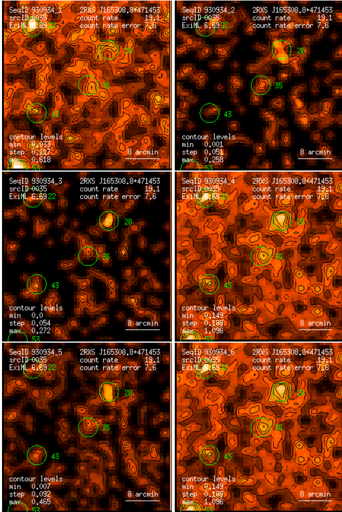
Figure 35: RASS 930934: detection 0035: band rate images, Gaussian filter: (1) PSPC channels 11 – 41, (2) 52 – 90, (3) 91 – 201, (4) 11 – 235, (5) 52 – 201, (6) 11 – 201. Broad band rates in counts/ks. Band rate contour levels in counts/ks/arcmin 2 .
