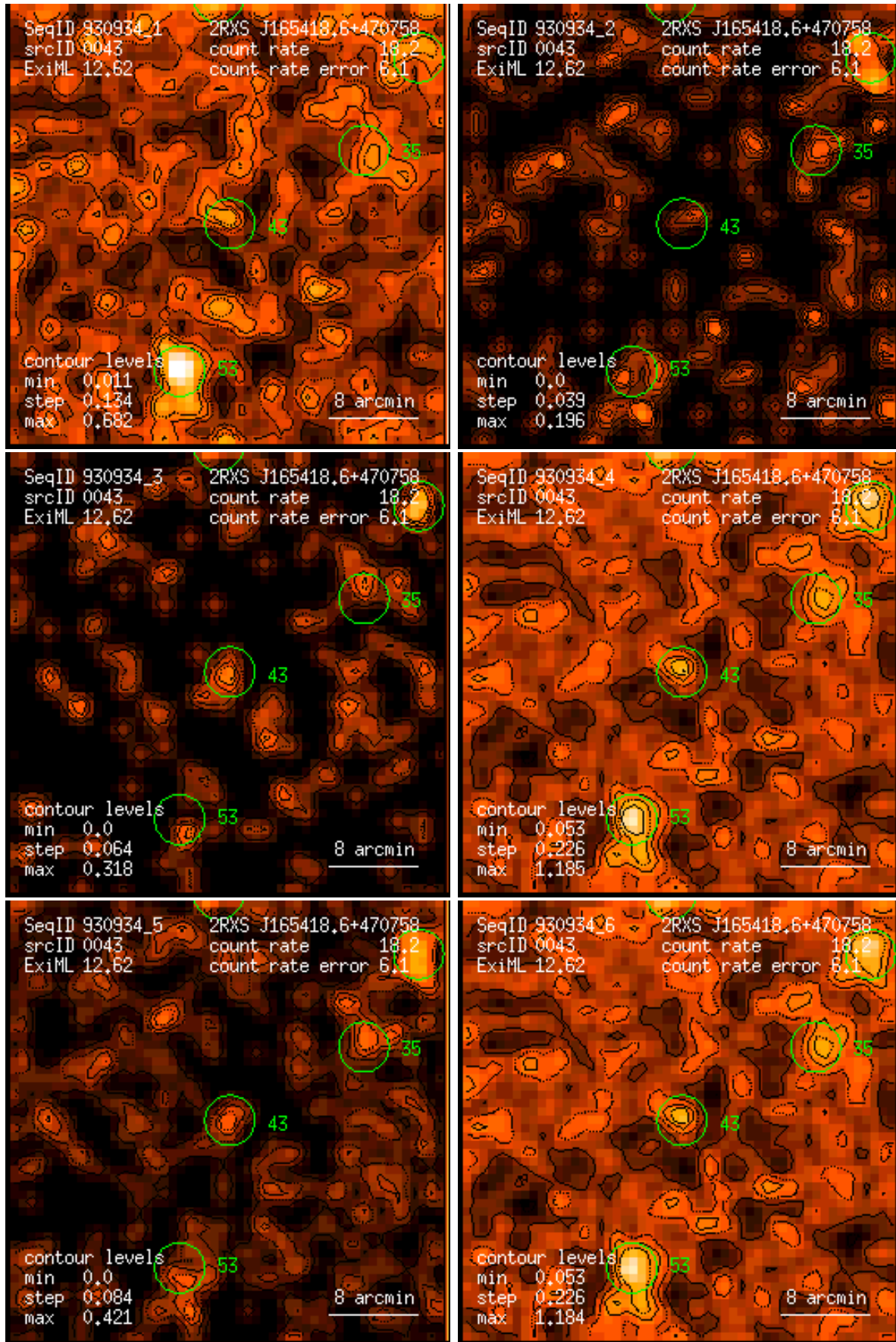
Figure 43: RASS 930934: detection 0043: band rate images, Gaussian filter: (1) PSPC channels 11 – 41, (2) 52 – 90, (3) 91 – 201, (4) 11 – 235, (5) 52 – 201, (6) 11 – 201. Broad band rates in counts/ks. Band rate contour levels in counts/ks/arcmin 2 .
