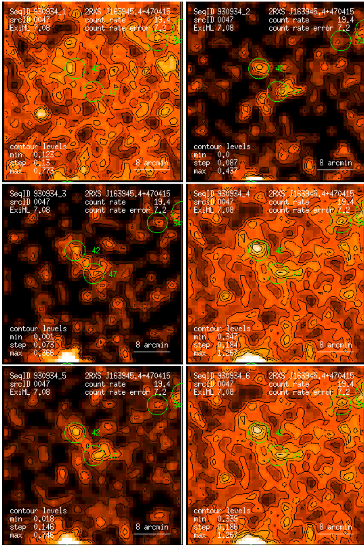
Figure 47: RASS 930934: detection 0047: band rate images, Gaussian filter: (1) PSPC channels 11 – 41, (2) 52 – 90, (3) 91 – 201, (4) 11 – 235, (5) 52 – 201, (6) 11 – 201. Broad band rates in counts/ks. Band rate contour levels in counts/ks/arcmin 2 .
