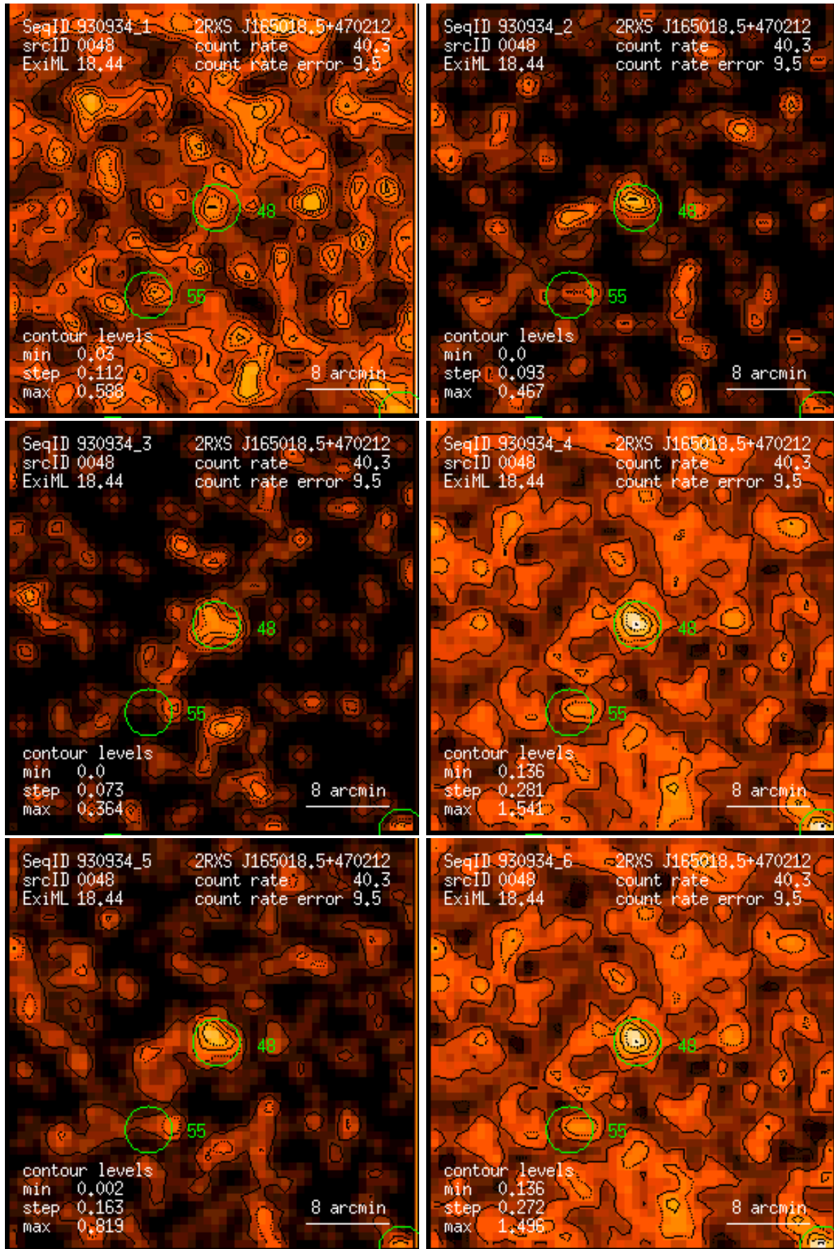
Figure 48: RASS 930934: detection 0048: band rate images, Gaussian filter: (1) PSPC channels 11 – 41, (2) 52 – 90, (3) 91 – 201, (4) 11 – 235, (5) 52 – 201, (6) 11 – 201. Broad band rates in counts/ks. Band rate contour levels in counts/ks/arcmin 2 .
