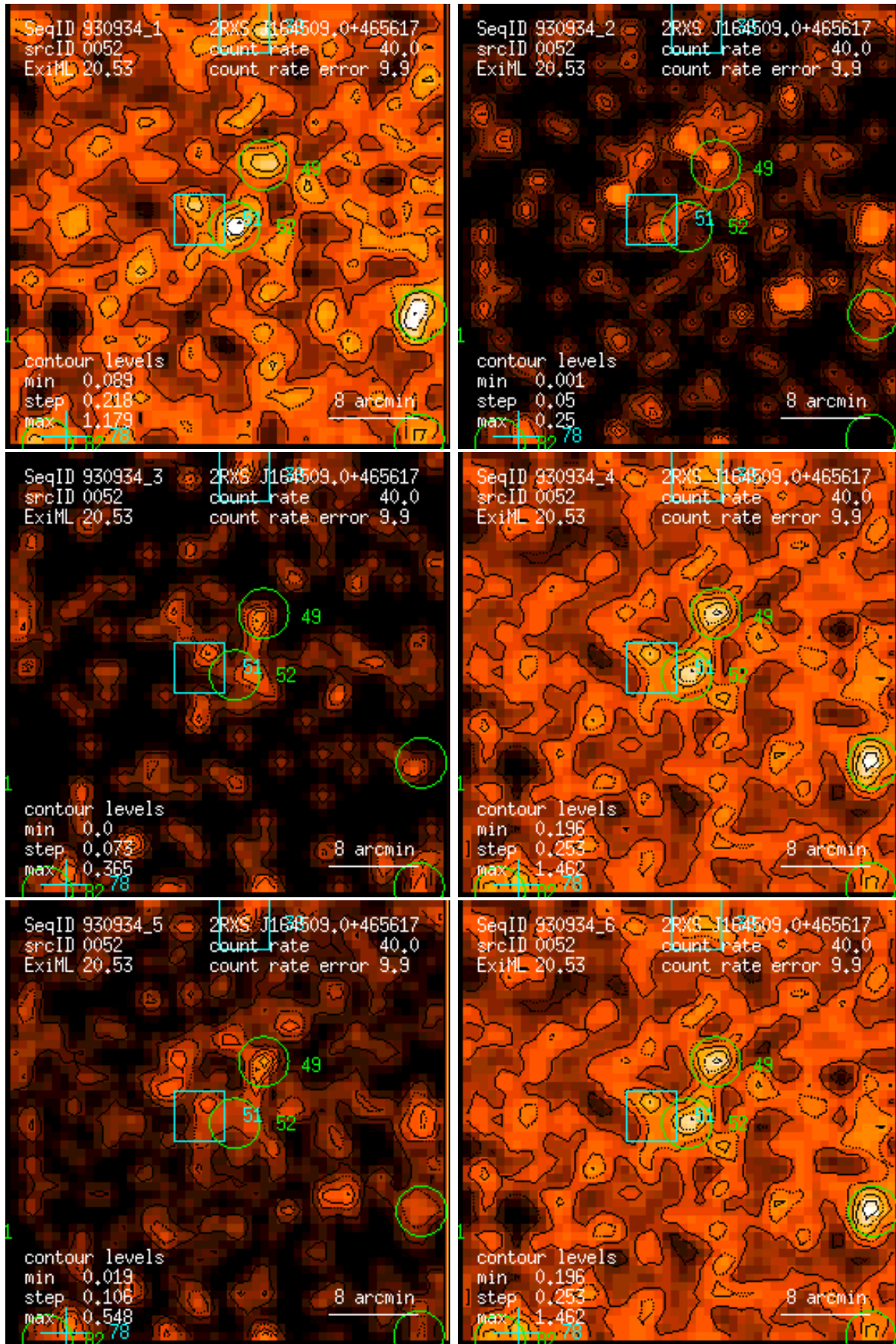
Figure 52: RASS 930934: detection 0052: band rate images, Gaussian filter: (1) PSPC channels 11 – 41, (2) 52 – 90, (3) 91 – 201, (4) 11 – 235, (5) 52 – 201, (6) 11 – 201. Broad band rates in counts/ks. Band rate contour levels in counts/ks/arcmin 2 .
