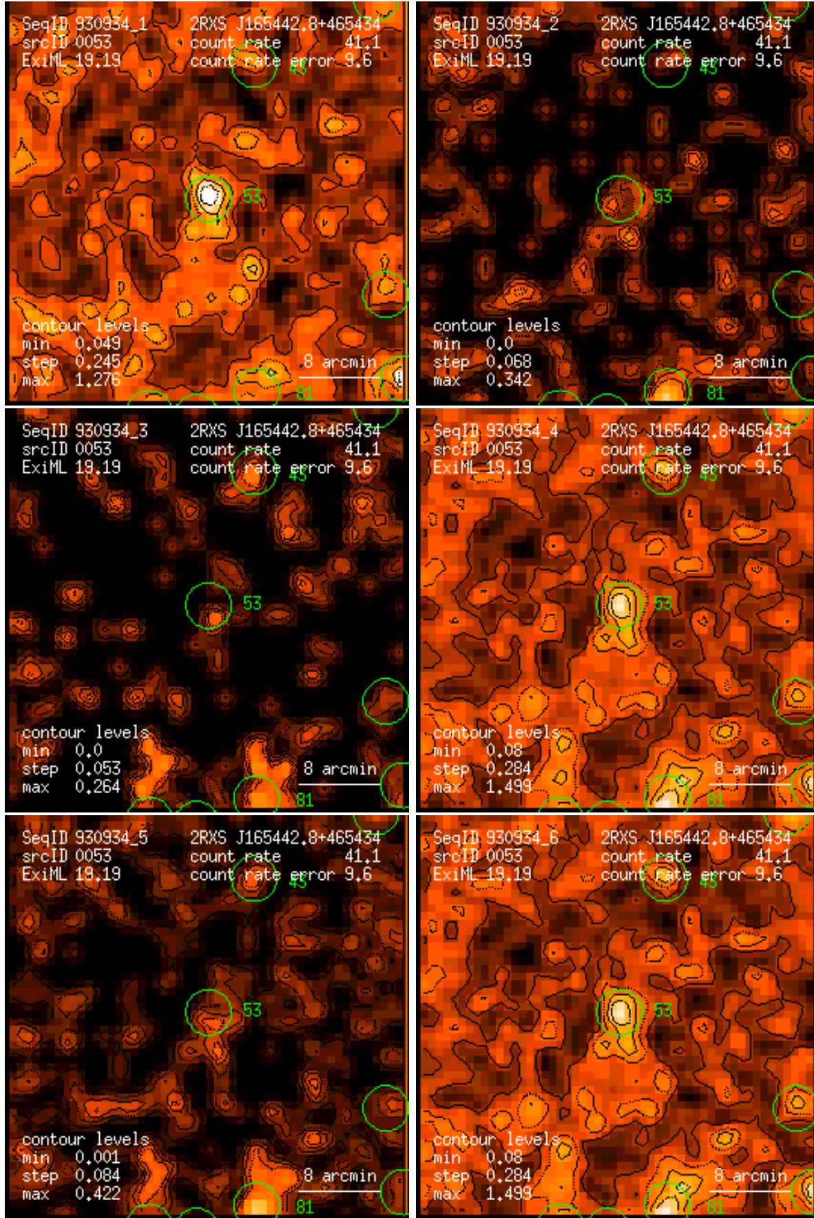
Figure 53: RASS 930934: detection 0053: band rate images, Gaussian filter: (1) PSPC channels 11 – 41, (2) 52 – 90, (3) 91 – 201, (4) 11 – 235, (5) 52 – 201, (6) 11 – 201. Broad band rates in counts/ks. Band rate contour levels in counts/ks/arcmin 2 .
