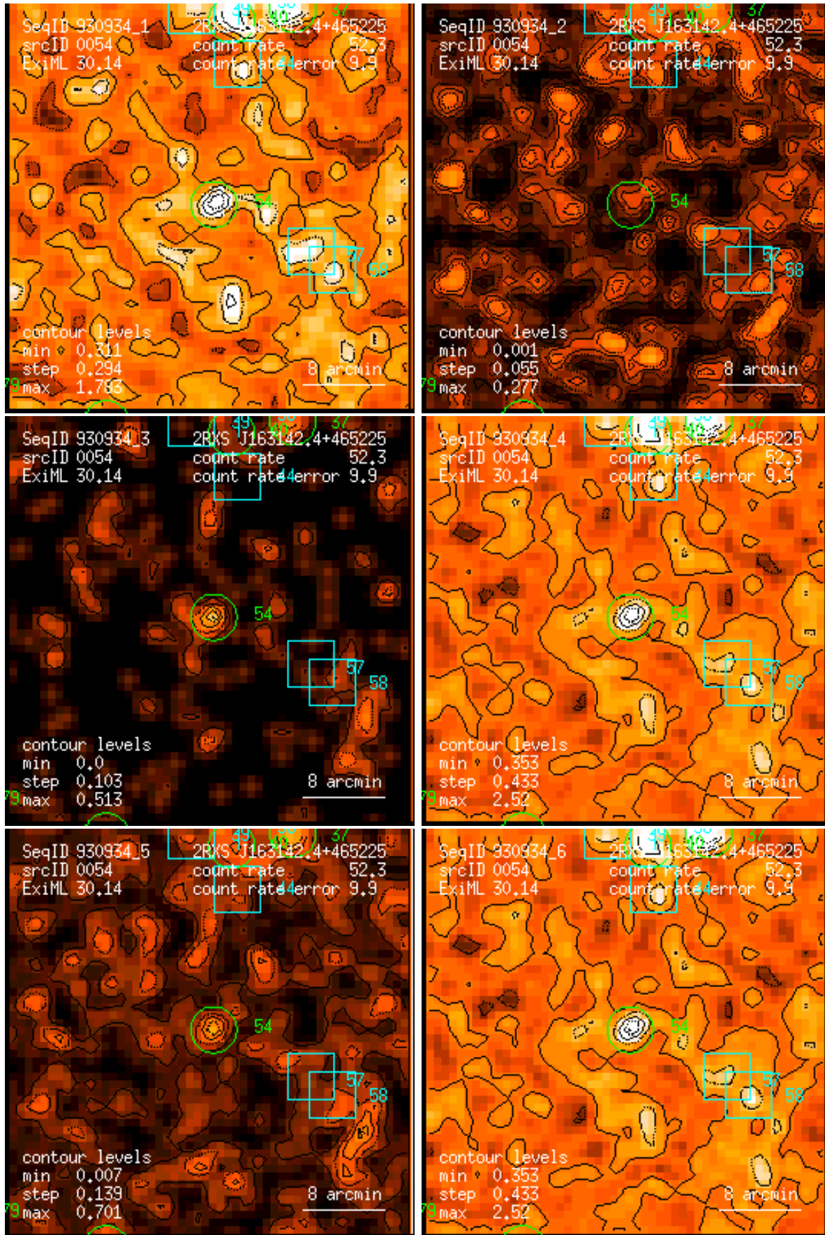
Figure 54: RASS 930934: detection 0054: band rate images, Gaussian filter: (1) PSPC channels 11 – 41, (2) 52 – 90, (3) 91 – 201, (4) 11 – 235, (5) 52 – 201, (6) 11 – 201. Broad band rates in counts/ks. Band rate contour levels in counts/ks/arcmin 2 .
