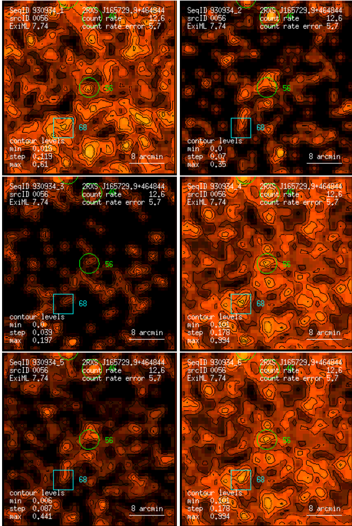
Figure 56: RASS 930934: detection 0056: band rate images, Gaussian filter: (1) PSPC channels 11 – 41, (2) 52 – 90, (3) 91 – 201, (4) 11 – 235, (5) 52 – 201, (6) 11 – 201. Broad band rates in counts/ks. Band rate contour levels in counts/ks/arcmin 2 .
