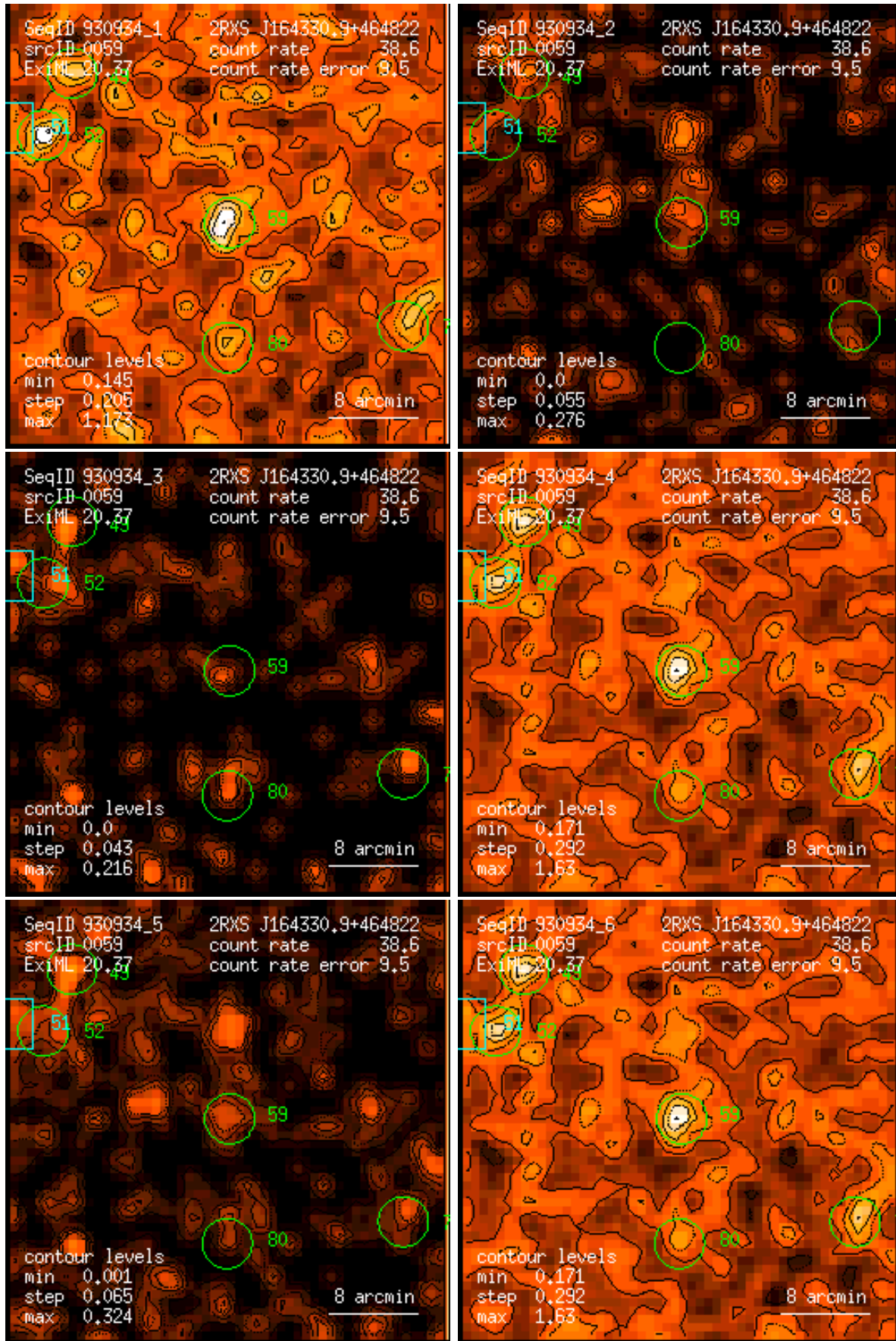
Figure 59: RASS 930934: detection 0059: band rate images, Gaussian filter: (1) PSPC channels 11 – 41, (2) 52 – 90, (3) 91 – 201, (4) 11 – 235, (5) 52 – 201, (6) 11 – 201. Broad band rates in counts/ks. Band rate contour levels in counts/ks/arcmin 2 .
