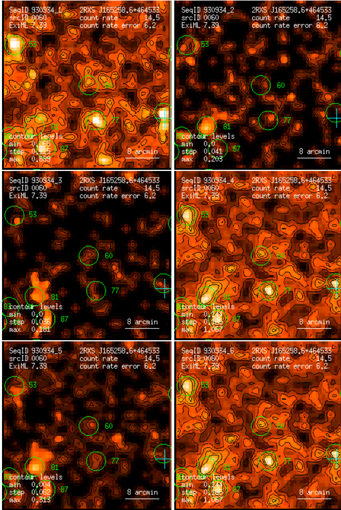
Figure 60: RASS 930934: detection 0060: band rate images, Gaussian filter: (1) PSPC channels 11 – 41, (2) 52 – 90, (3) 91 – 201, (4) 11 – 235, (5) 52 – 201, (6) 11 – 201. Broad band rates in counts/ks. Band rate contour levels in counts/ks/arcmin 2 .
